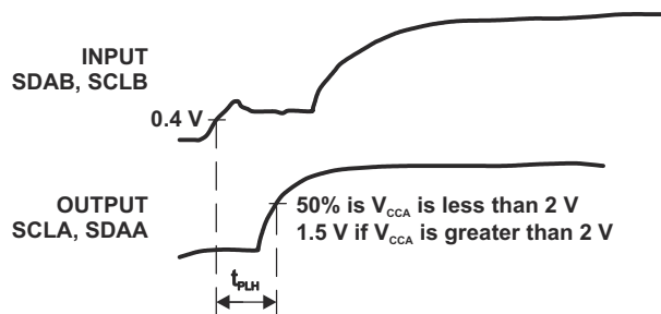
图 6-4. Waveform 3 - Propagation Delay for B-side to A-side
