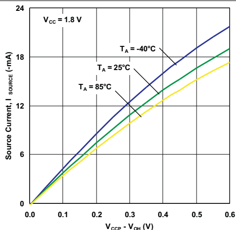
Figure 11. I/O Source Current vs Output High Voltage ( V_{CC} = 1.8\text{ V} )
