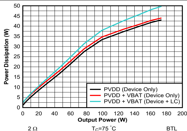
图 7-11. Power Dissipation vs Output Power - 14.4 V - 2 \Omega
