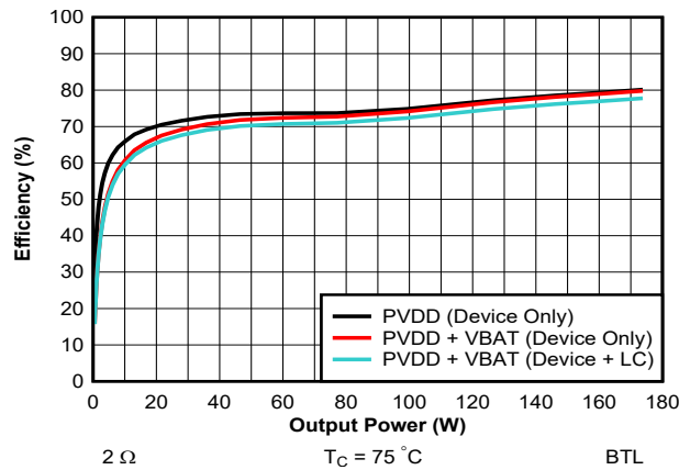
图 7-9. Efficiency vs Output Power - 14.4 V - 2 \Omega
