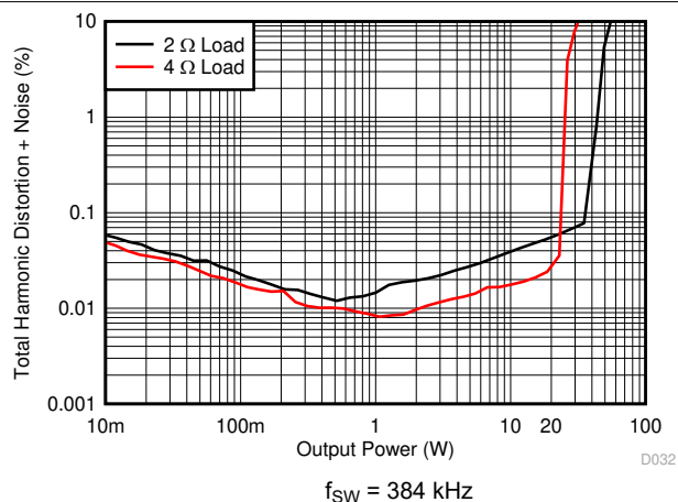
图 7-20. PBTL THD+N vs Power
