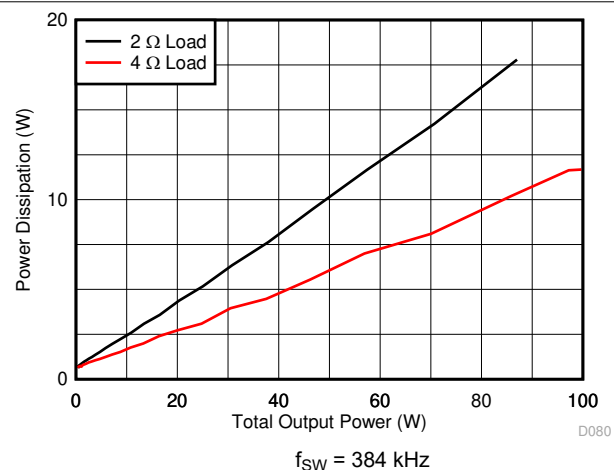
图 7-24. Power Dissipation vs Total Output Power
