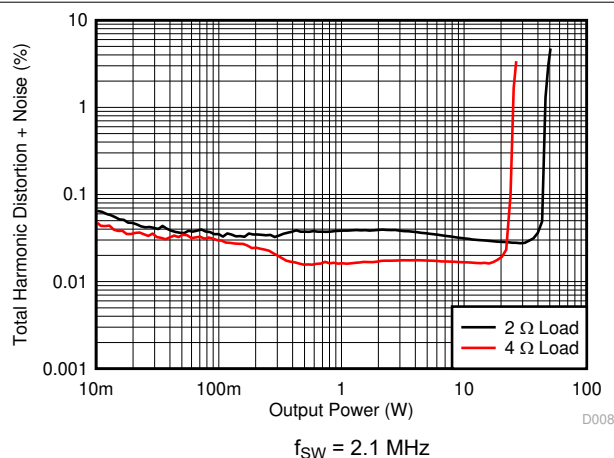
图 7-21. PBTL THD+N vs Power
