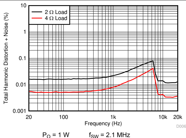
图 7-5. THD+N vs Frequency
