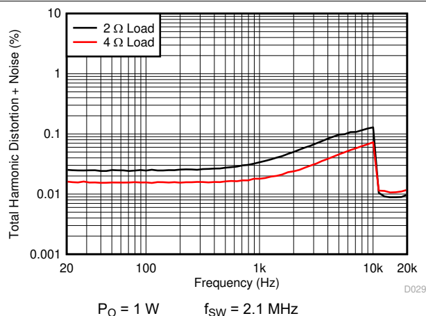
图 7-19. PBTL THD+N vs Frequency
