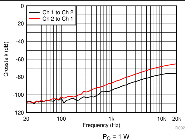
图 7-1. Crosstalk vs Frequency
