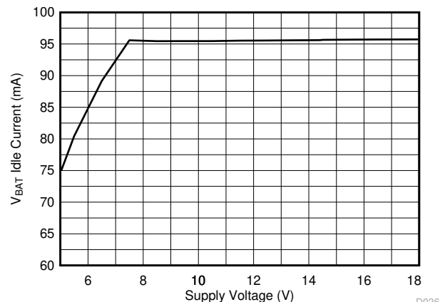
图 7-16. VBAT Idle Current vs Voltage
