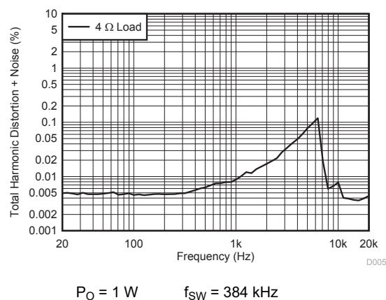
图 7-4. THD+N vs Frequency
