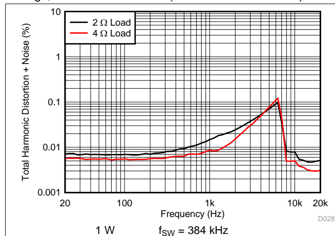
图 19. PBTL THD+N vs Frequency
