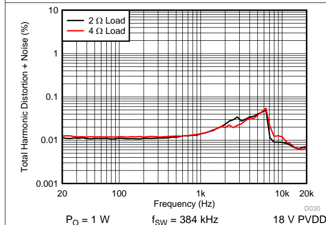
图 21. PBTL THD+N vs Frequency
