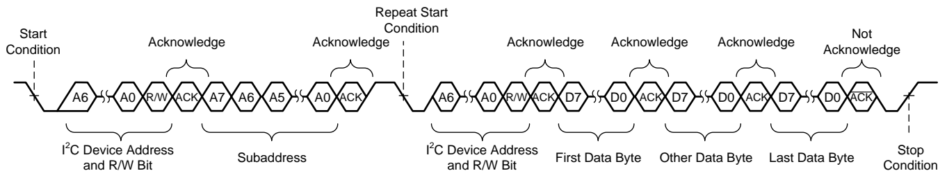
图 46. Sequential Read Transfer
