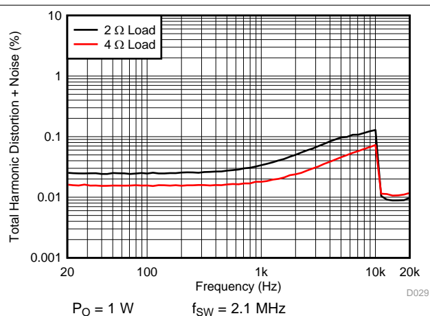
图 20. PBTL THD+N vs Frequency
