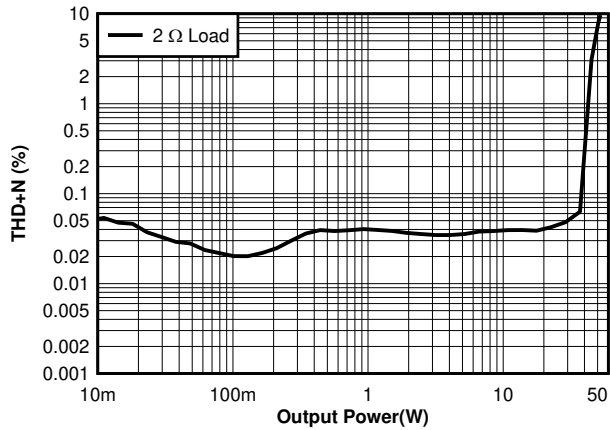
图 7-28. THD+N vs Power - PBTL - 14.4V
