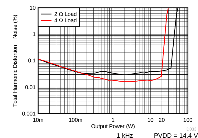
图 83. THD vs Output Power, 2R
