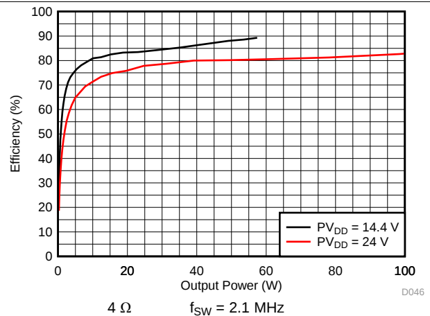
图 16. PVDD Power Efficiency vs Total Output Power
