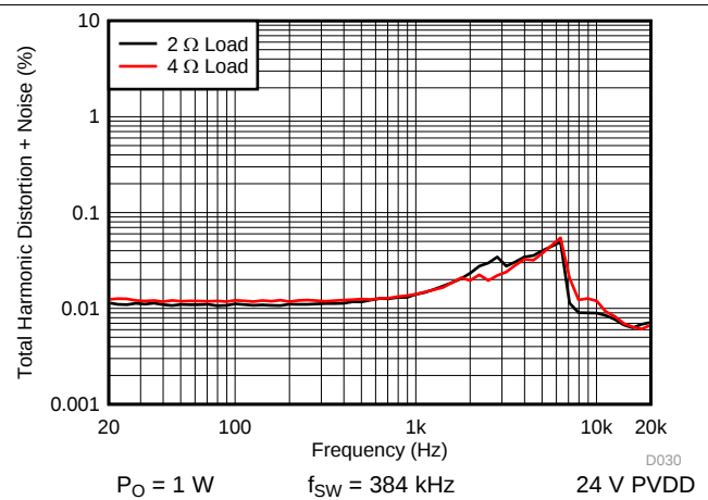
图 24. PBTL THD+N vs Frequency
