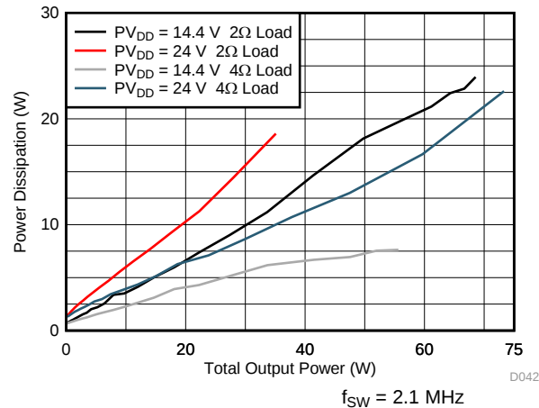
图 33. Power Dissipation vs Total Output Power
