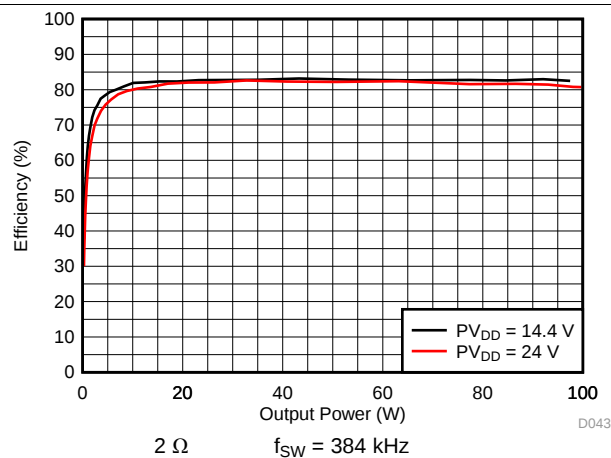
图 17. PVDD Power Efficiency vs Total Output Power
