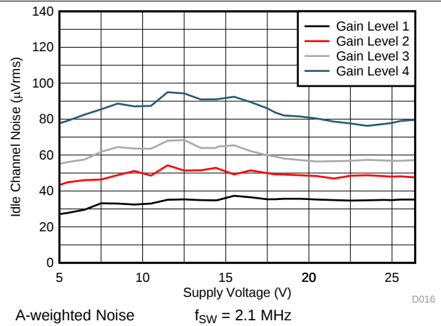
图 14. Noise vs Supply voltage
