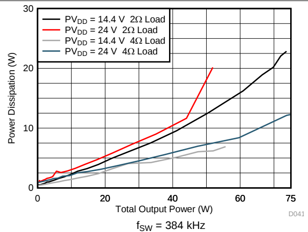
图 32. Power Dissipation vs Total Output Power
