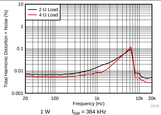
图 22. PBTL THD+N vs Frequency
