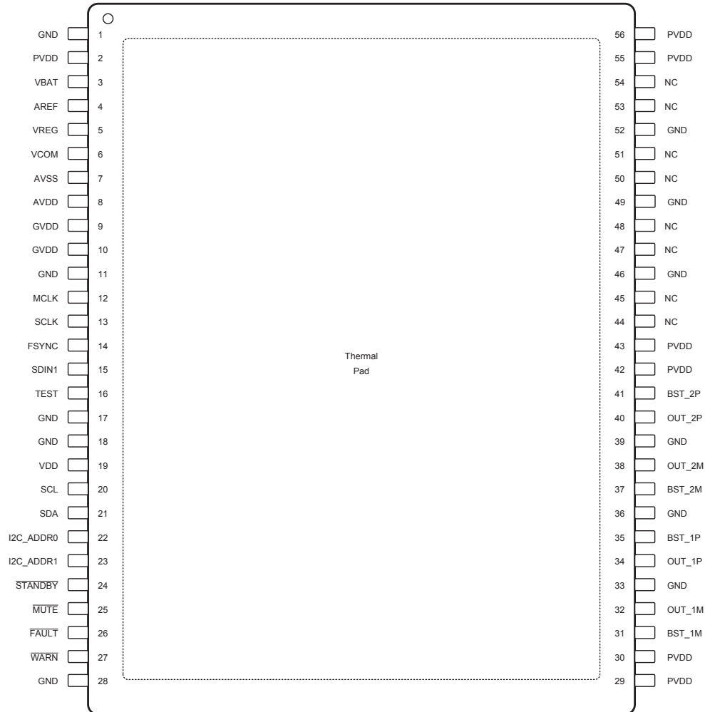
Pin Functions
