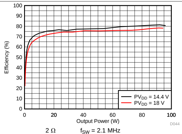
图 18. PVDD Power Efficiency vs Total Output Power
