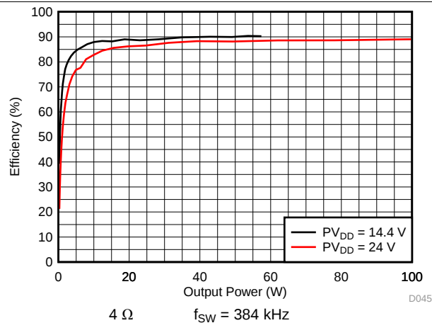
图 15. PVDD Power Efficiency vs Total Output Power
