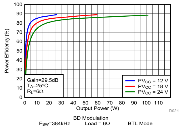
图 6-18. Efficiency vs Output Power
