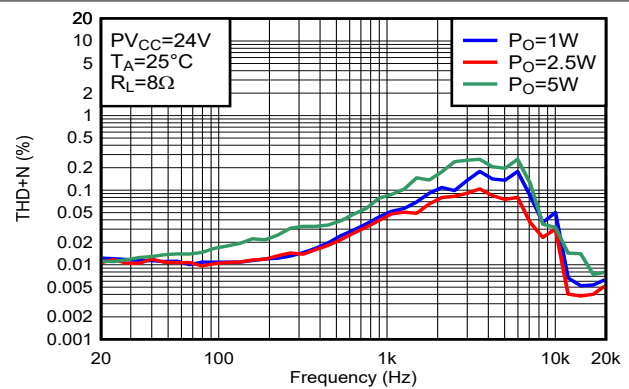
图 6-23. THD+N vs Frequency-BTL
