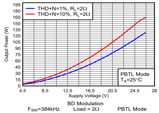
图 6-48. Output Power vs Supply Voltage
