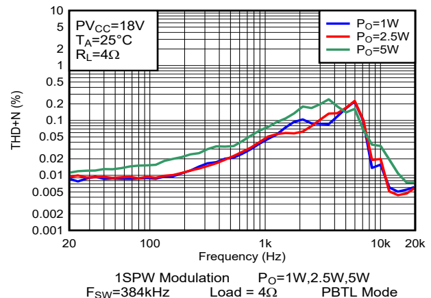
图 6-59. THD+N vs Frequency-PBTL
