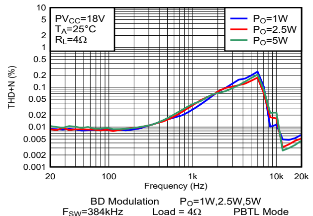
图 6-42. THD+N vs Frequency-PBTL
