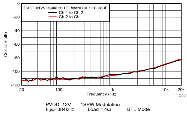
图 6-34. Crosstalk
