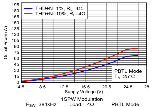
图 6-67. Output Power vs Supply Voltage
