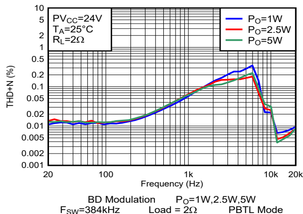
图 6-43. THD+N vs Frequency-PBTL
