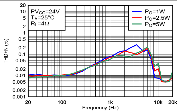
图 6-22. THD+N vs Frequency-BTL
