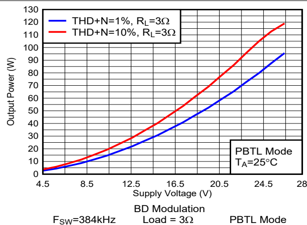
图 6-49. Output Power vs Supply Voltage
