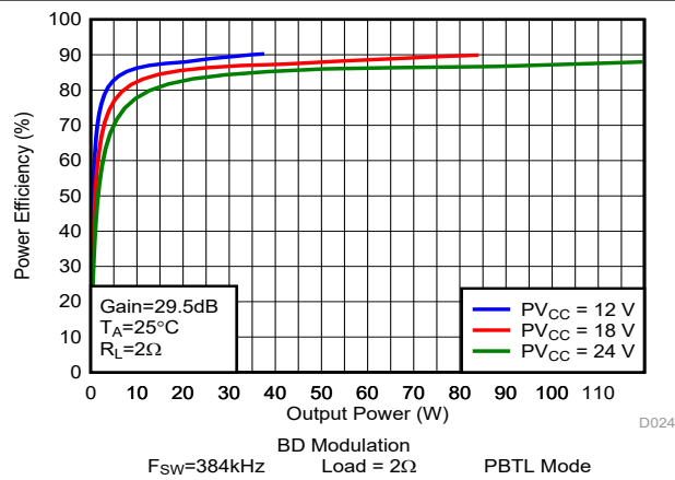
图 6-53. Efficiency vs Output Power
