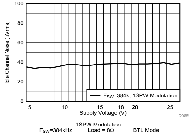
图 6-33. Idle Channel Noise vs Supply Voltage
