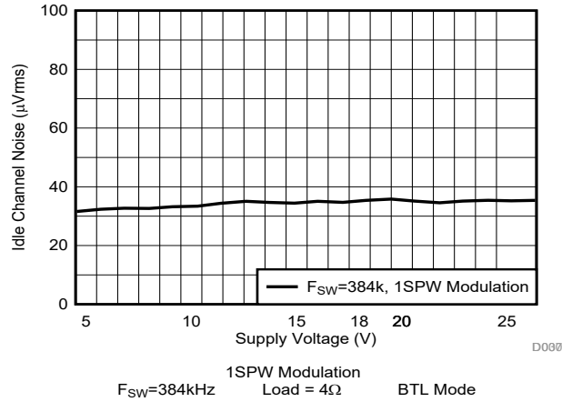
图 6-32. Idle Channel Noise vs Supply Voltage
