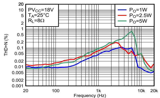
图 6-21. THD+N vs Frequency-BTL
