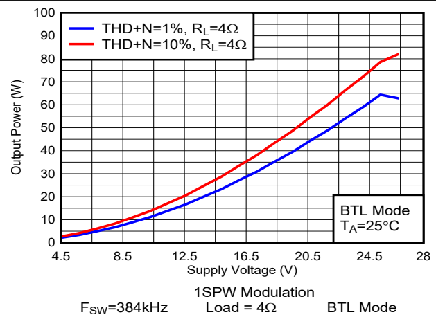
图 6-29. Output Power vs Supply Voltage
