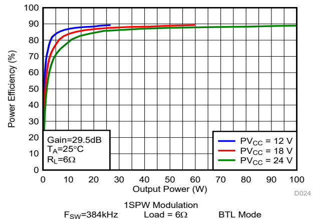
图 6-37. Efficiency vs Output Power
