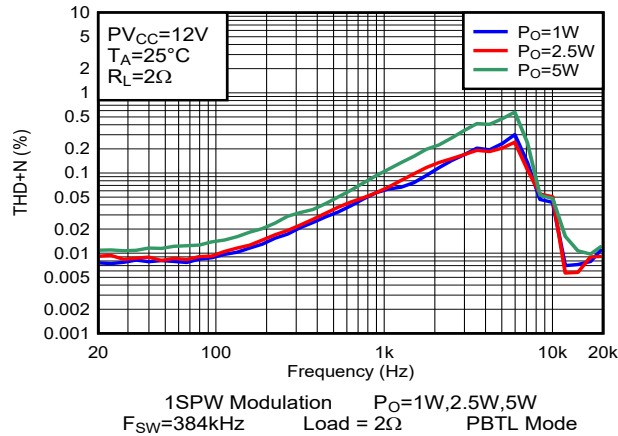
图 6-56. THD+N vs Frequency-PBTL
