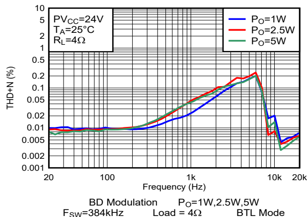
图 6-5. THD+N vs Frequency-BTL
