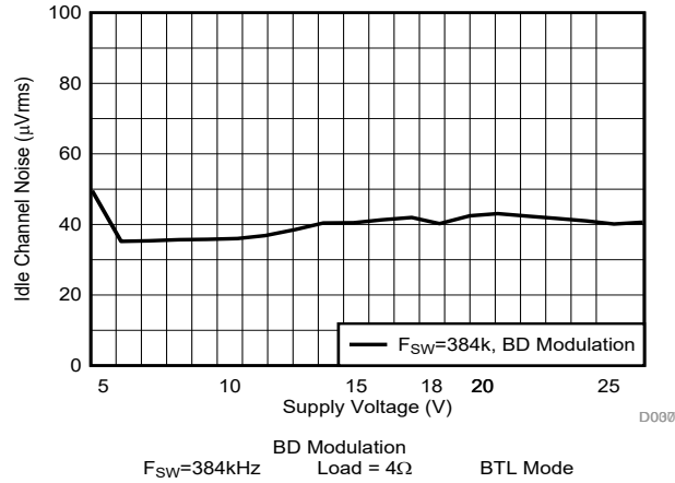
图 6-13. Idle Channel Noise vs Supply Voltage
