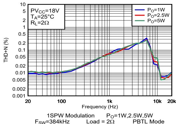
图 6-58. THD+N vs Frequency-PBTL
