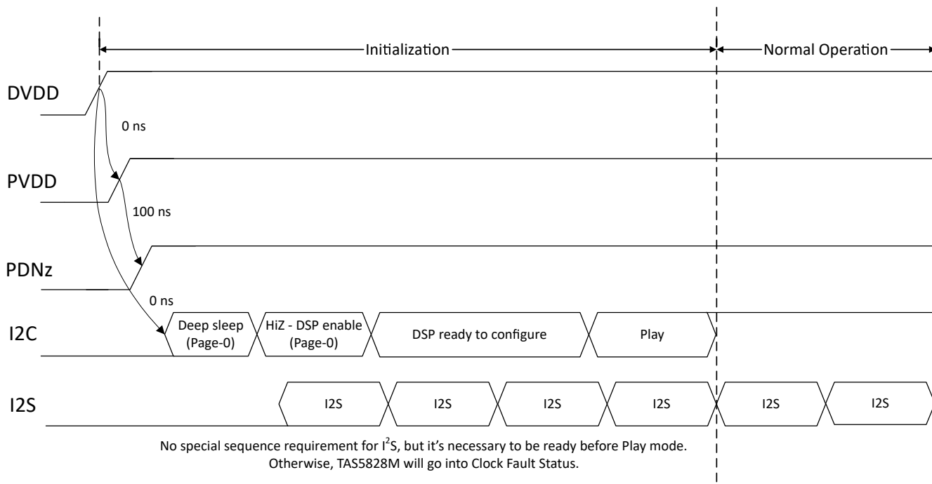
图 8-16. TAS5828M Startup Sequence
