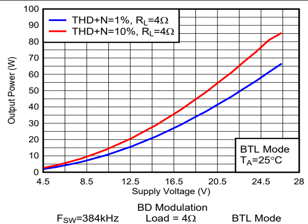
图 6-10. Output Power vs Supply Voltage
