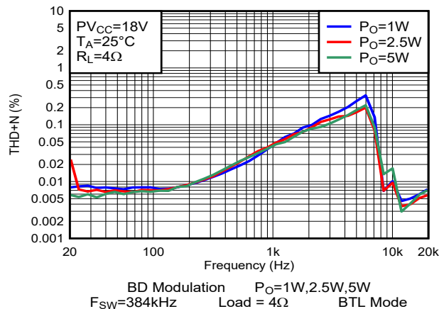
图 6-3. THD+N vs Frequency-BTL
