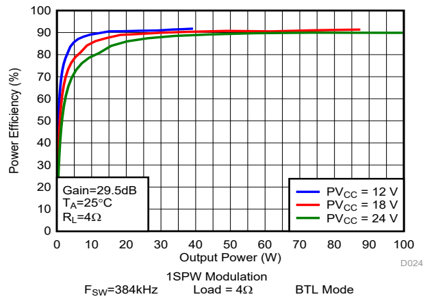
图 6-36. Efficiency vs Output Power
