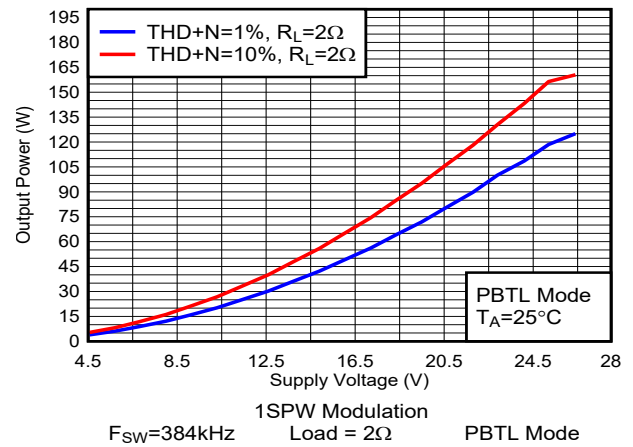
图 6-65. Output Power vs Supply Voltage
