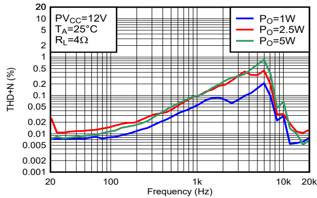
图 6-20. THD+N vs Frequency-BTL
