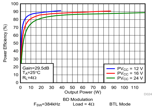
图 6-17. Efficiency vs Output Power
