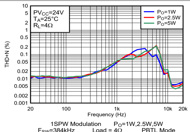
图 6-61. THD+N vs Frequency-PBTL
