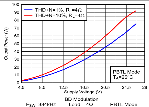
图 6-50. Output Power vs Supply Voltage
