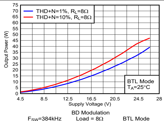
图 6-12. Output Power vs Supply Voltage
