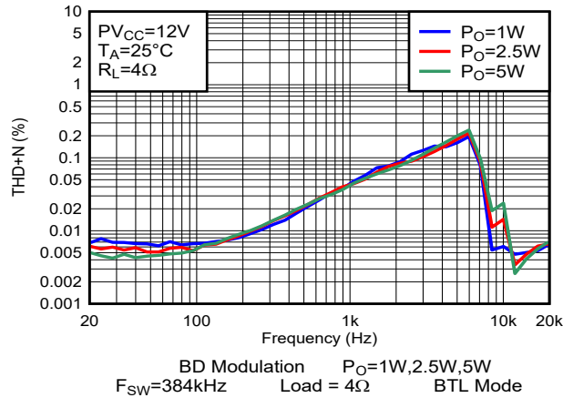
图 6-1. THD+N vs Frequency-BTL
