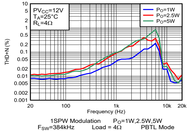
图 6-57. THD+N vs Frequency-PBTL
