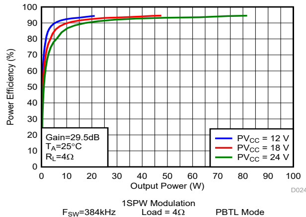
图 6-72. Efficiency vs Output Power
