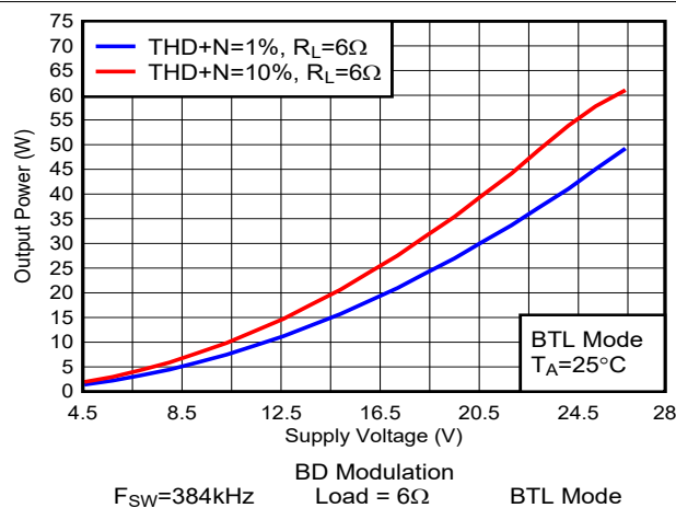
图 6-11. Output Power vs Supply Voltage
