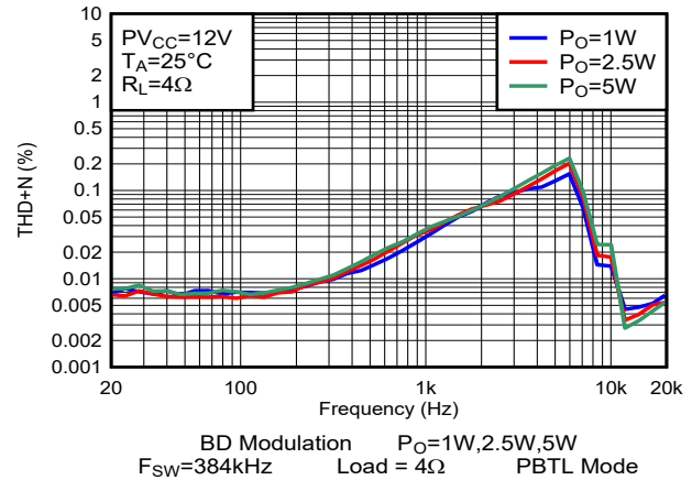
图 6-40. THD+N vs Frequency-PBTL
