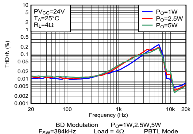
图 6-44. THD+N vs Frequency-PBTL
