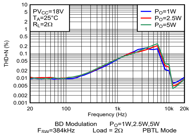
图 6-41. THD+N vs Frequency-PBTL
