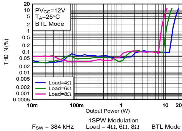
图 6-26. THD+N vs Output Power-BTL
