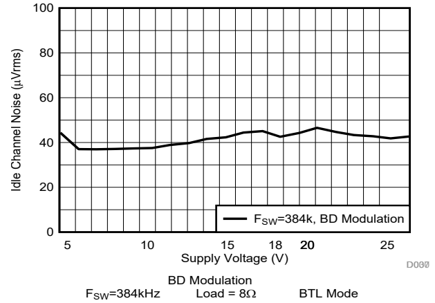
图 6-14. Idle Channel Noise vs Supply Voltage
