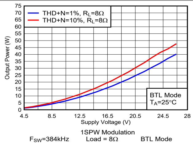
图 6-31. Output Power vs Supply Voltage
