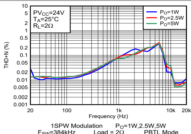
图 6-60. THD+N vs Frequency-PBTL
