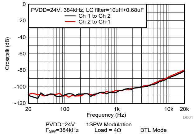
图 6-35. Crosstalk - old
