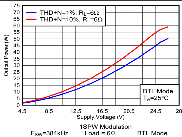
图 6-30. Output Power vs Supply Voltage
