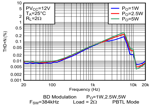
图 6-39. THD+N vs Frequency-PBTL
