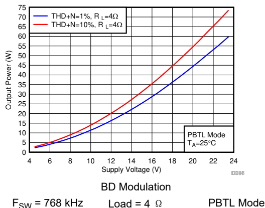
图 7-74. Output Power vs Supply Voltage
