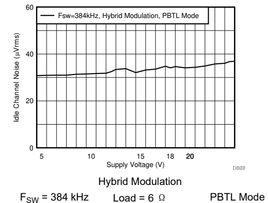
图 7-34. Idle Channel Noise vs Supply Voltage
