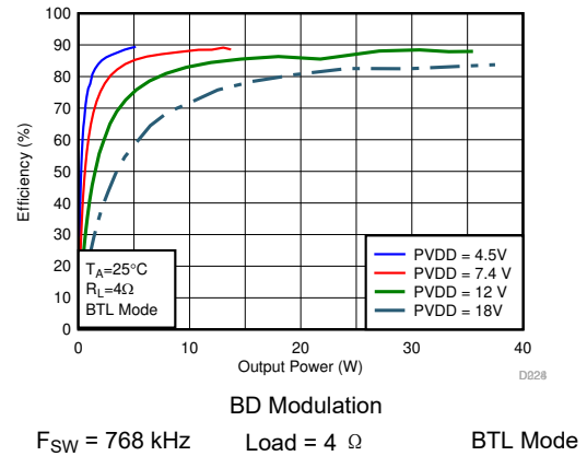
图 7-61. Efficiency vs Output Power
