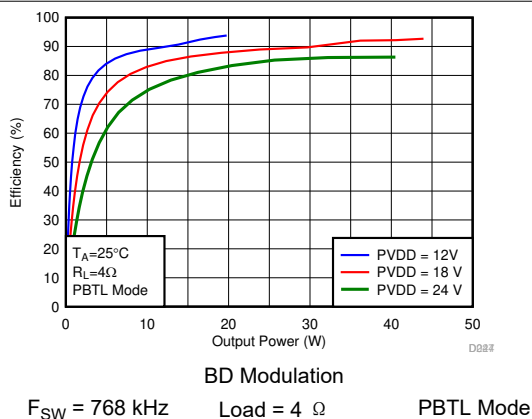
图 7-76. Efficiency vs Output Power
