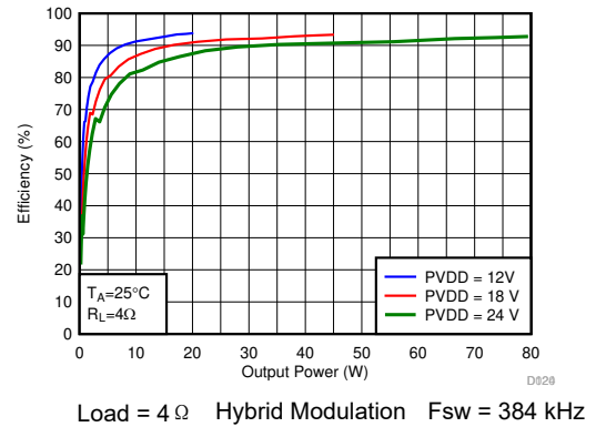
图 10-11. Efficiency vs Output Power
