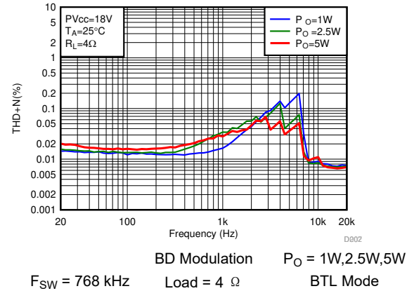
图 7-43. THD+N vs Frequency-BTL
