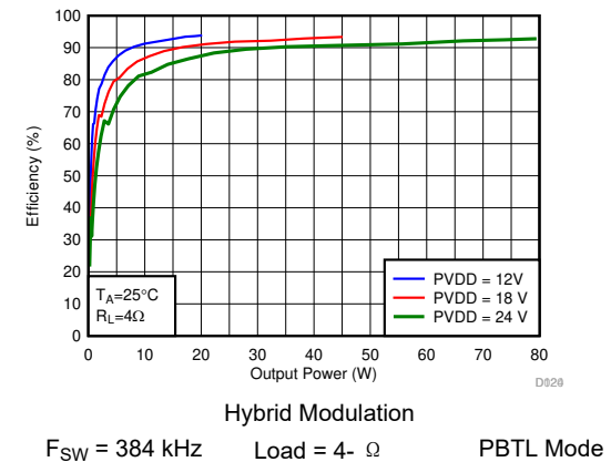
图 7-32. Efficiency vs Output Power
