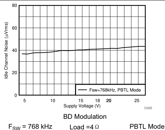
图 7-77. Idle Channel Noise vs Supply Voltage
