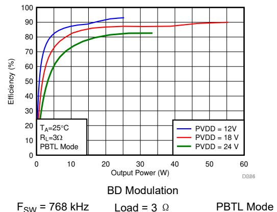
图 7-75. Efficiency vs Output Power
