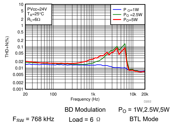
图 7-47. THD+N vs Frequency-BTL
