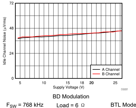
图 7-58. Idle Channel Noise vs Supply Voltage
