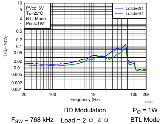
图 7-36. THD+N vs Frequency-BTL
