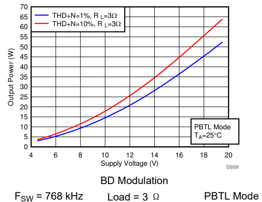
图 7-73. Output Power vs Supply Voltage
