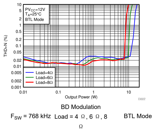
图 7-50. THD+N vs Output Power-BTL
