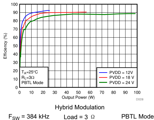
图 7-33. Efficiency vs Output Power
