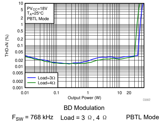
图 7-71. THD+N vs Output Power-PBTL
