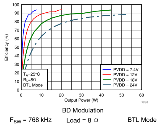
图 7-63. Efficiency vs Output Power
