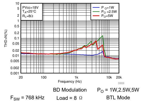
图 7-45. THD+N vs Frequency-BTL
