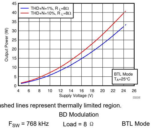
图 7-57. Output Power vs Supply Voltage
