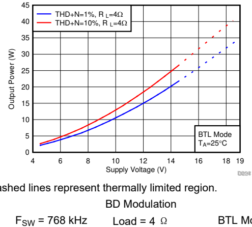
图 7-55. Output Power vs Supply Voltage
