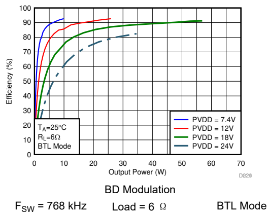
图 7-62. Efficiency vs Output Power
