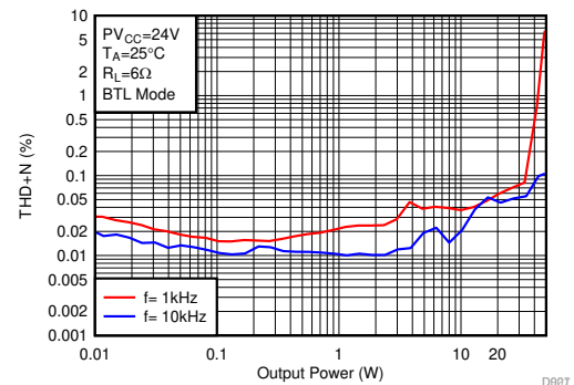
图 6-12. THD+N vs Output Power-BTL
