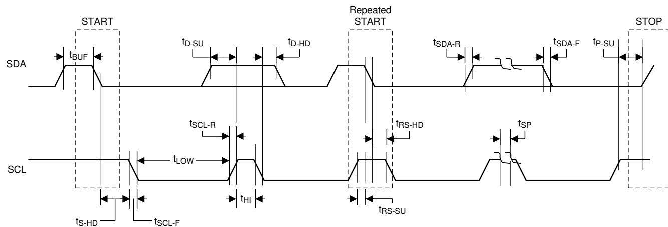
图 6-2. I²C Communication Port Timing Diagram
