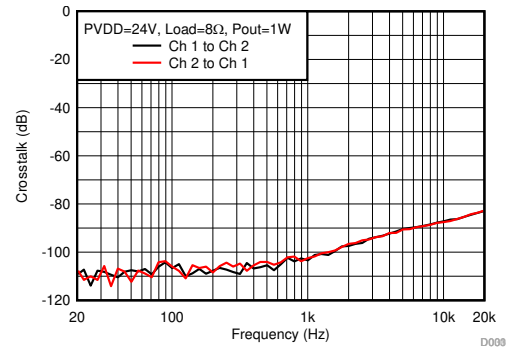
图 6-30. Crosstalk vs Frequency-BTL
