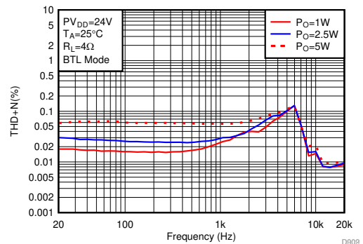
图 6-18. THD+N vs Frequency-BTL
