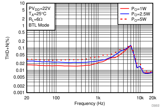
图 6-22. THD+N vs Frequency-BTL
