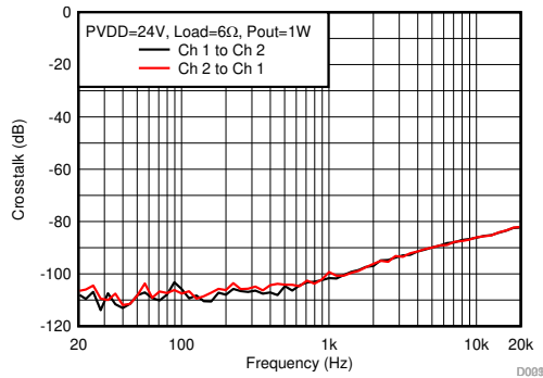
图 6-29. Crosstalk vs Frequency-BTL
