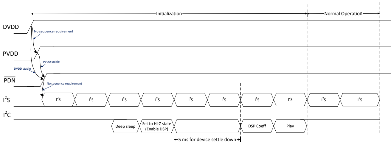
图 7-15. Startup sequence
