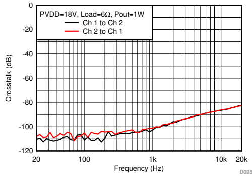
图 6-27. Crosstalk vs Frequency-BTL
