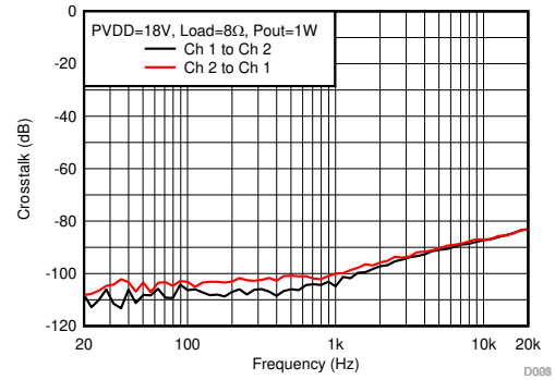
图 6-28. Crosstalk vs Frequency-BTL
