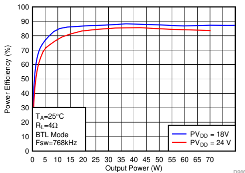
图 6-3. Efficiency vs Output Power-BTL
