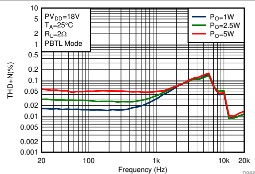
图 6-52. THD+N vs Frequency
