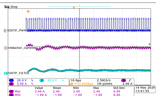
图 8-4. Start-up Current (Fsw = 768 kHz, LC filter = 4.7 \mu H + 0.68 \mu F, PVDD = 24 V, 1SPW Modulation)
