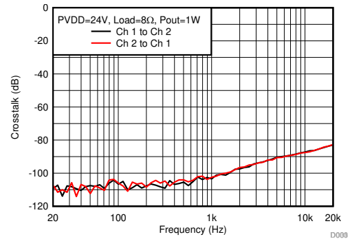
图 6-30. Crosstalk vs Frequency-BTL
