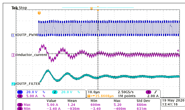
图 8-3. Start-up Current (Fsw = 768 kHz, LC filter = 4.7 \mu H + 0.68 \mu F, PVDD = 24 V, BD Modulation)
