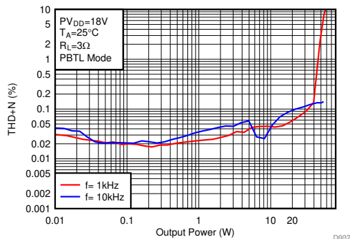
图 6-39. THD+N vs Output Power
