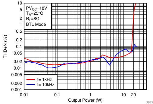
图 6-15. THD+N vs Output Power-BTL
