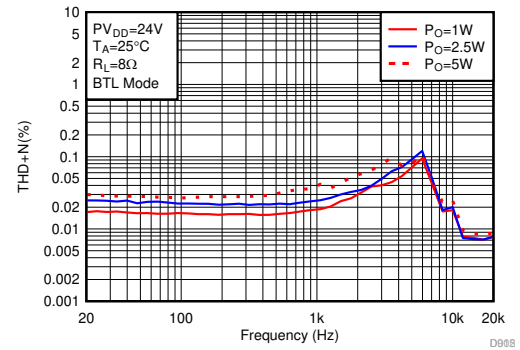
图 6-24. THD+N vs Frequency-BTL
