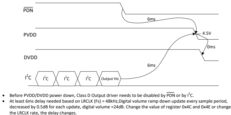
图 7-15. Power-Down Sequence
