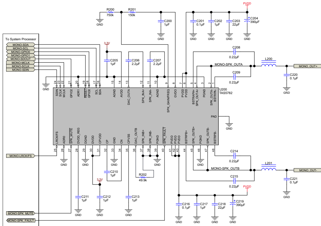
图 81. Mono (PBTTL) System Application Schematic
