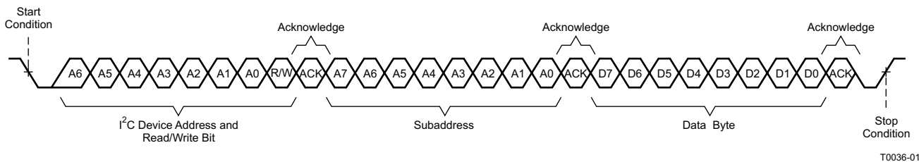
Figure 10. Write Transfer
