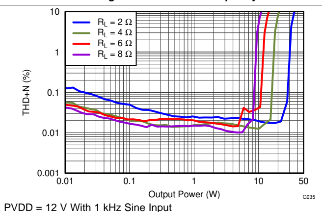
Figure 31. THD+N vs Output Power
