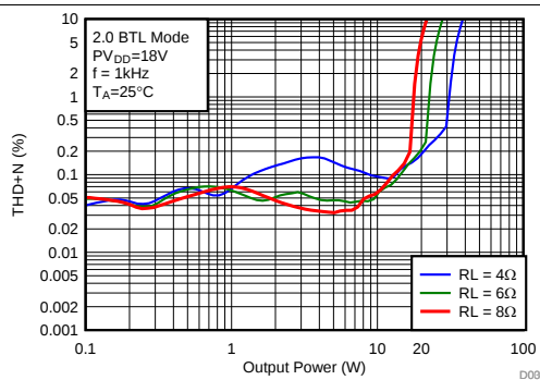
图 20. Total Harmonic Distortion + Noise vs Output Power
