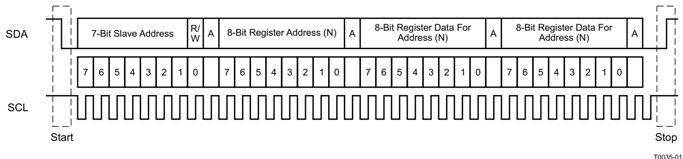
图 60. Typical I²C Sequence
