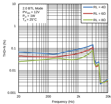
图 22. Total Harmonic Distortion vs Frequency
