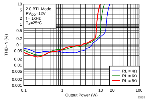
图 19. Total Harmonic Distortion + Noise vs Output Power
