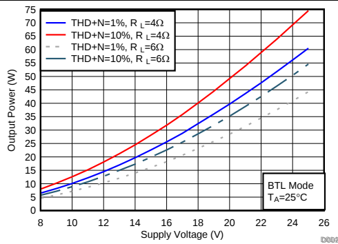
图 18. Output Power vs Supply Voltage
