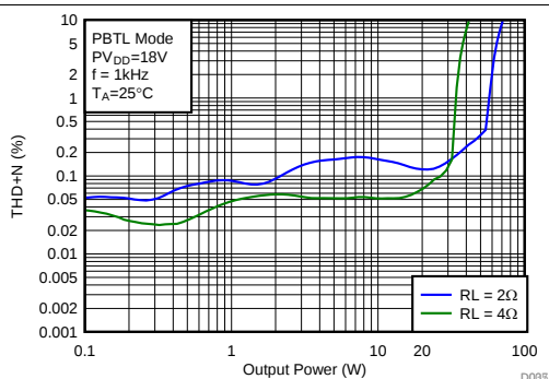
图 34. Total Harmonic Distortion + Noise vs Output Power (PBTL Mode)
