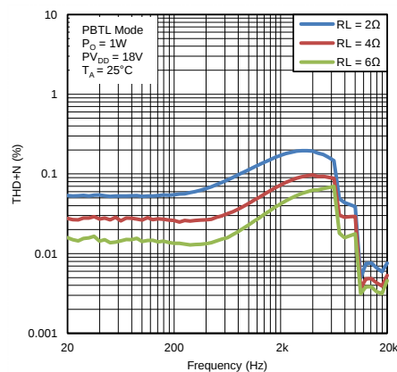
图 37. Total Harmonic Distortion vs Frequency (PBTL Mode)
