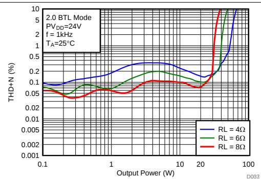
图 21. Total Harmonic Distortion + Noise vs Output Power
