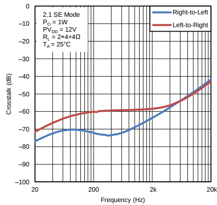
图 15. Crosstalk vs Frequency
