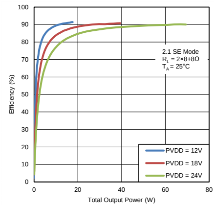
图 12. Efficiency vs Total Output Power
