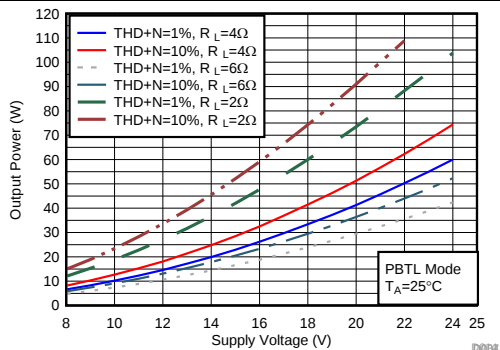
图 32. Output Power vs Supply Voltage
