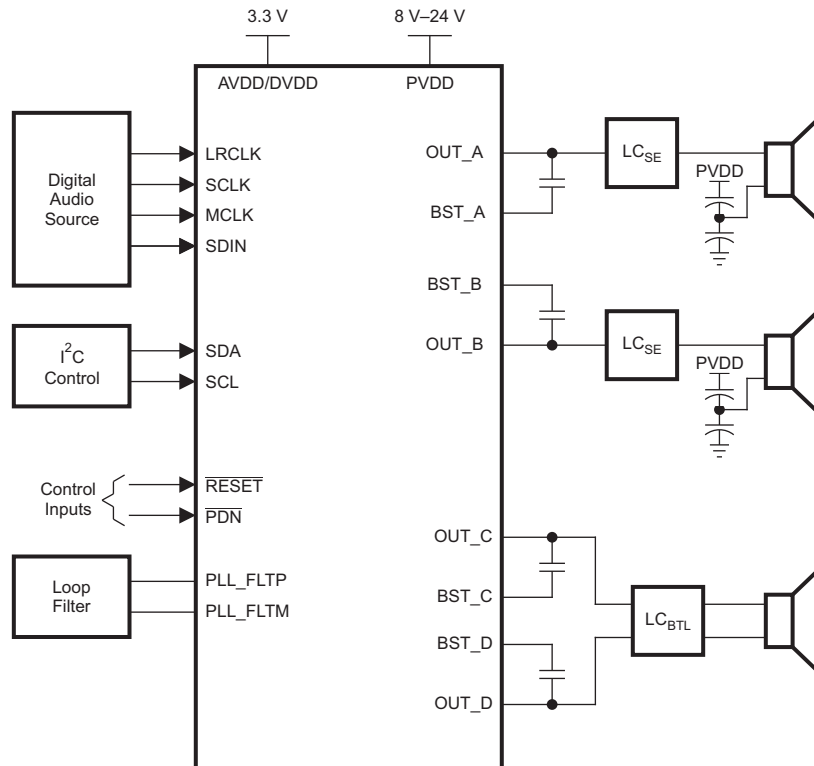
图 72. Simplified 2.1 Application Diagram
