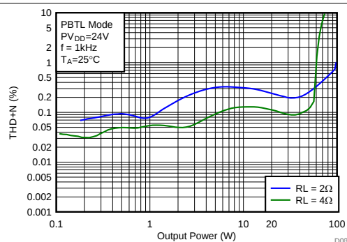
图 35. Total Harmonic Distortion + Noise vs Output Power (PBTL Mode)
