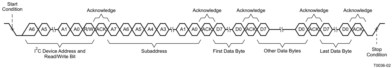
图 62. Multiple-Byte Write Transfer
