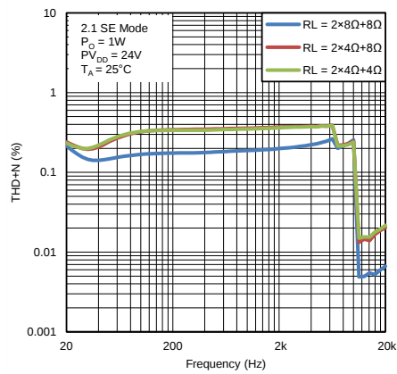
图 11. Total Harmonic Distortion + Noise vs Frequency
