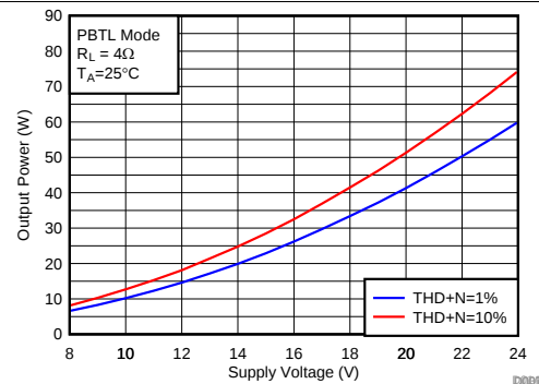
图 41. Power vs Supply Voltage (PBTL Mode)
