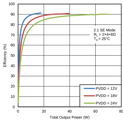
图 13. Efficiency vs Total Output Power
