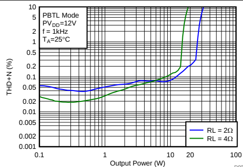
图 33. Total Harmonic Distortion + Noise vs Output Power (PBTL Mode)
