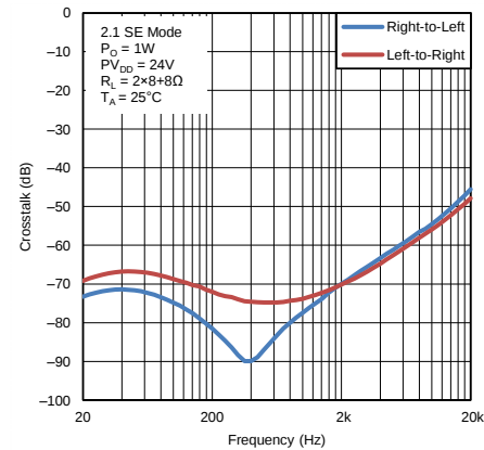
图 16. Crosstalk vs Frequency
