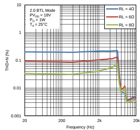
图 23. Total Harmonic Distortion vs Frequency
