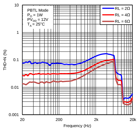
图 36. Total Harmonic Distortion vs Frequency (PBTL Mode)
