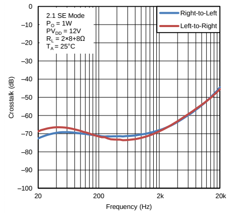
图 14. Crosstalk vs Frequency
