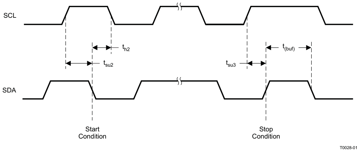
图 3. Start and Stop Conditions Timing
