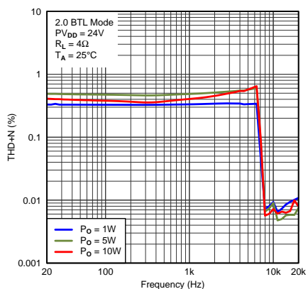
图 15. THD+N vs Frequency
