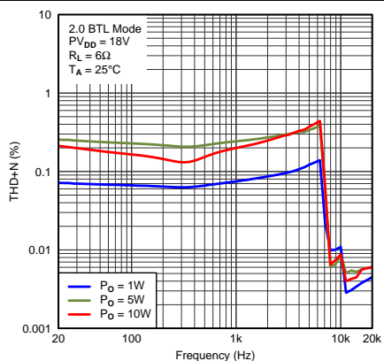
图 11. THD+N vs Frequency
