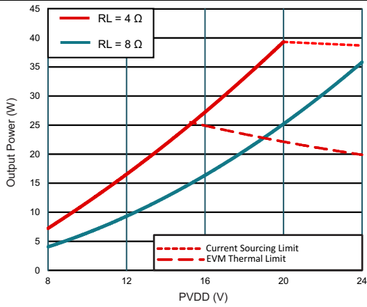
图 5. Output Power vs Supply Voltage
