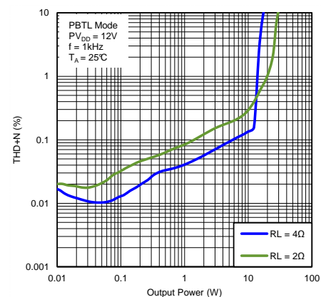
图 34. Total Harmonic Distortion + Noise vs Output Power (PBTL Mode)
