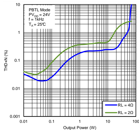
图 36. Total Harmonic Distortion + Noise vs Output Power (PBTL Mode)
