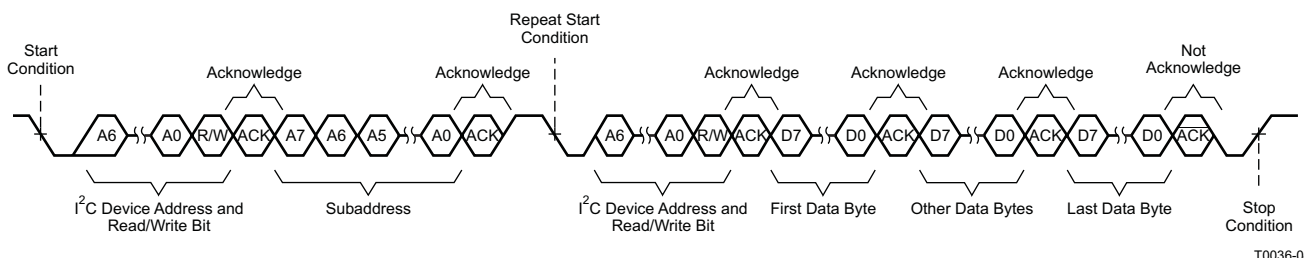
图 54. Multiple-Byte Read Transfer
