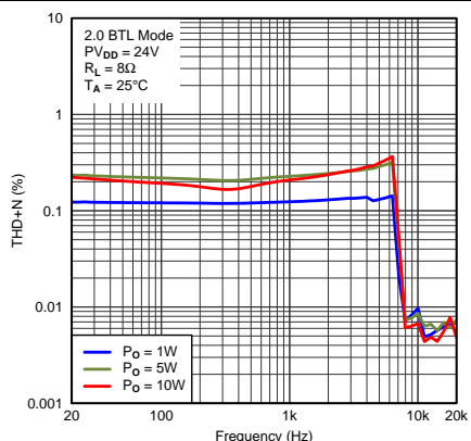
图 13. THD+N vs Frequency
