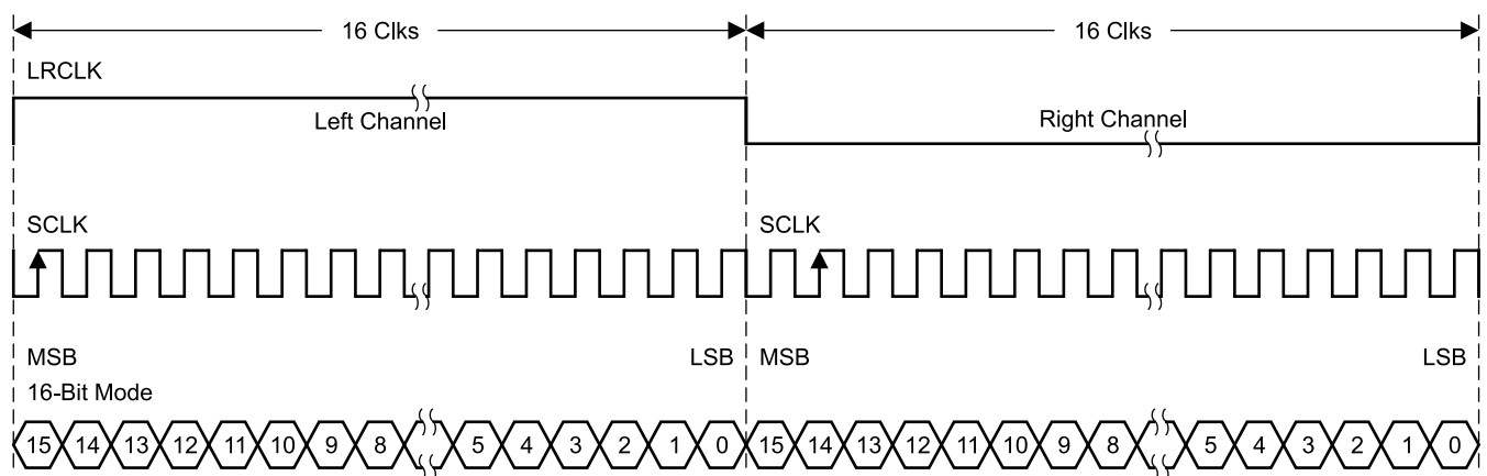
图 63. Right-Justified 32-f s Format
