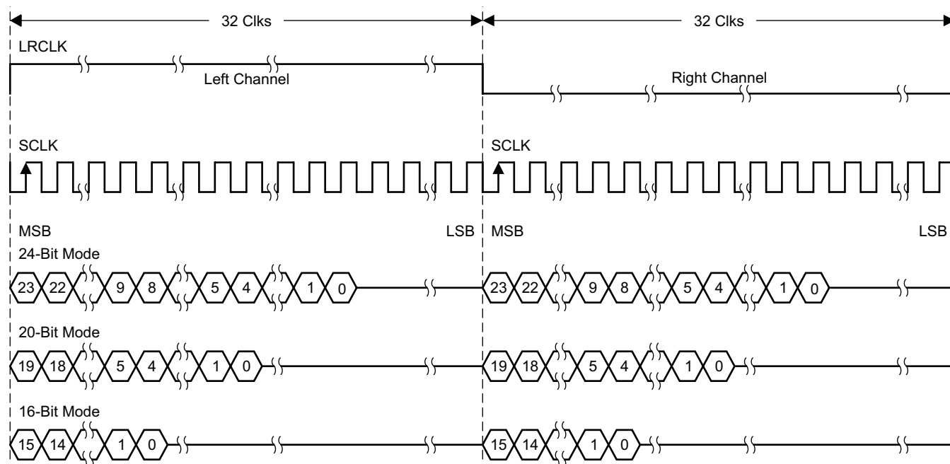
图 58. Left-Justified 64- f_s Format
