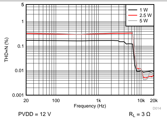
图 18. THD+N vs Frequency - PBTL
