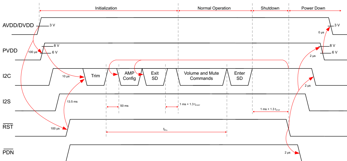
图 50. Recommended Start-Up and Shutdown Sequence
