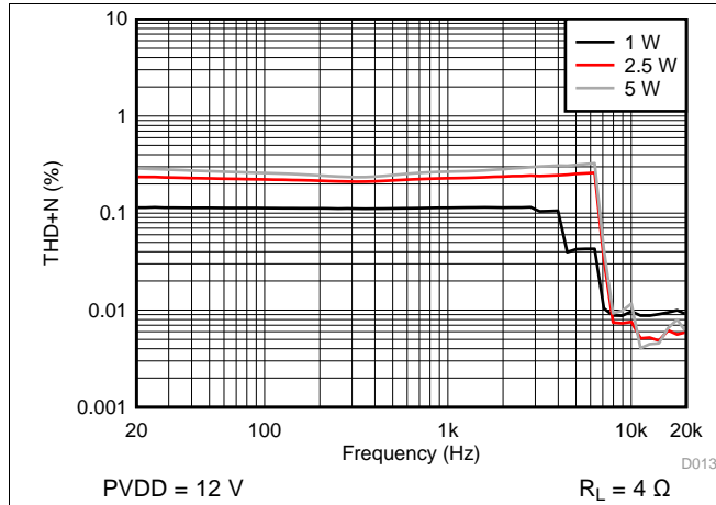
图 17. THD+N vs Frequency - PBTL
