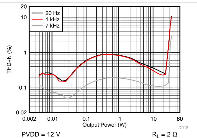
图 22. THD+N vs Output Power - PBTL
