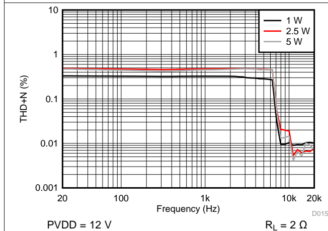
图 19. THD+N vs Frequency - PBTL
