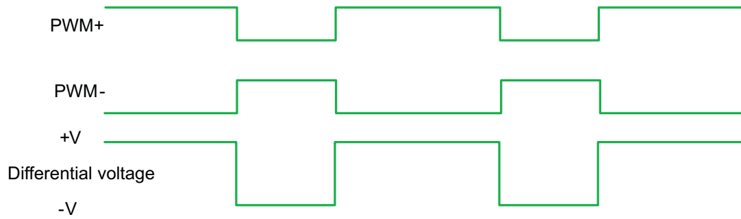
Figure 20. AD Modulation
