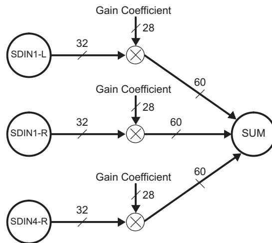
Figure 32. Input Crossbar Mixer
