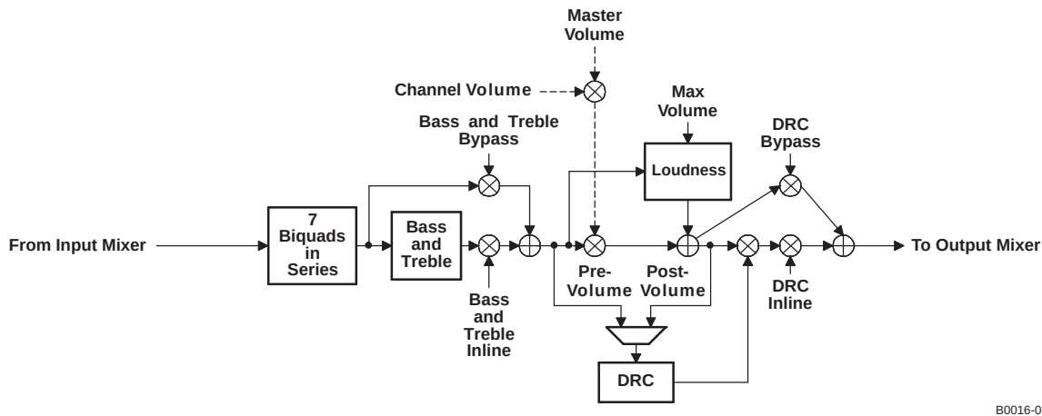
Figure 36. DRC Positioning in TAS5558 Processing Flow
