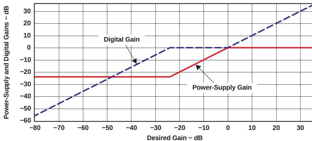
Figure 18. Power-Supply and Digital Gains (Linear Space)
