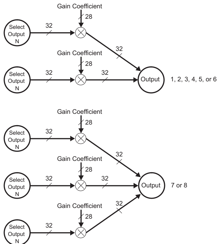
Figure 39. Output Mixers
