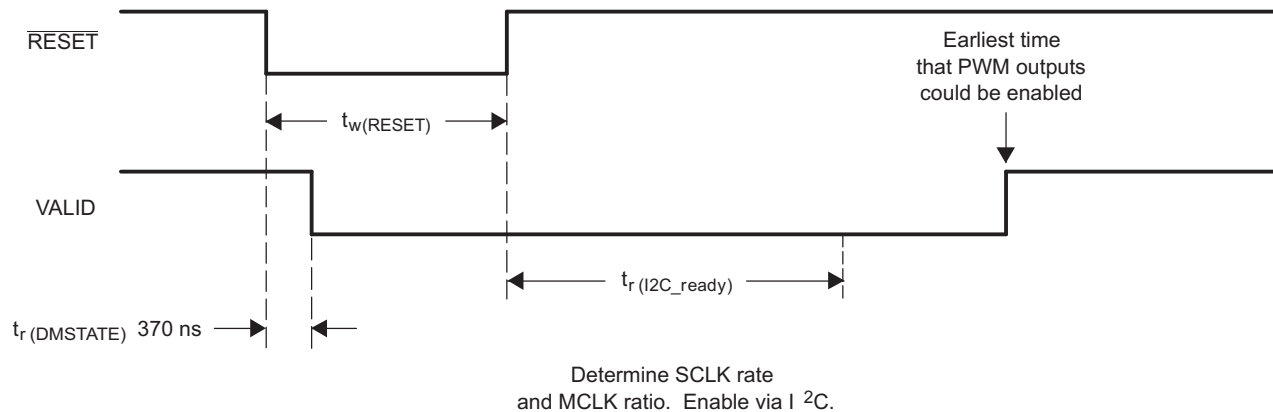
Figure 3. Reset Timing
