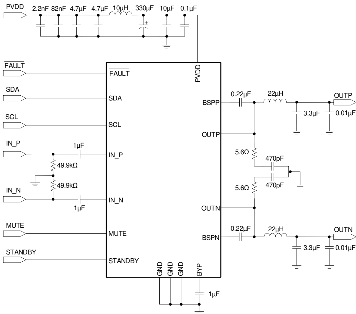
图 8-1. TAS5441-Q1 Typical Application Schematic
