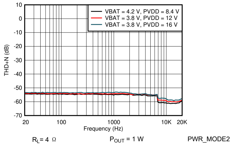
图 6-35. I Sense THDN vs Frequency
