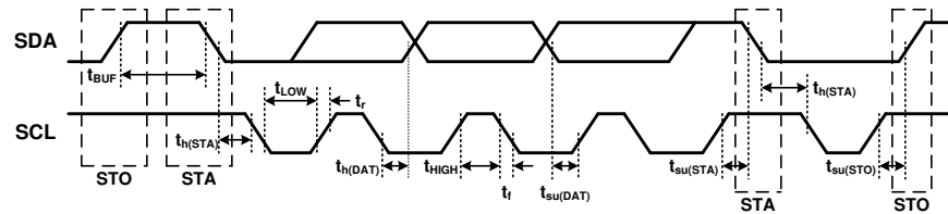
图 6-1. I2C Timing Diagram
