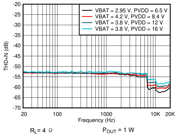
图 6-33. I Sense THDN vs Frequency
