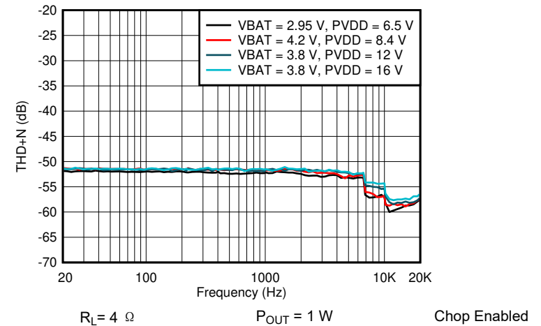
图 6-34. I Sense THDN vs Frequency
