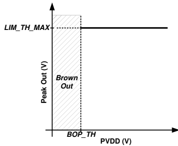
图 8-6. Limiter with Fixed Threshold
