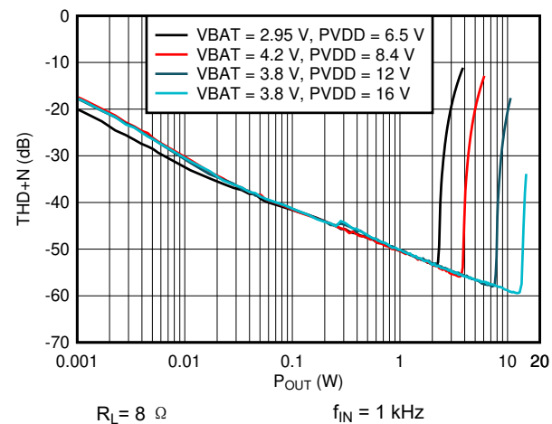
图 6-30. I Sense THDN vs Output Power
