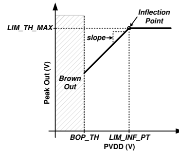
图 8-7. Limiter with Inflection Point
