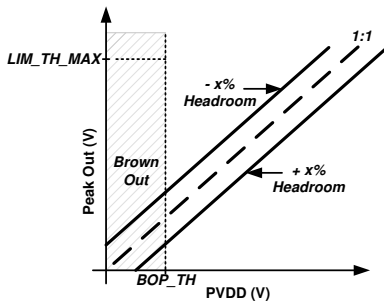
图 8-8. Limiter with Dynamic Threshold
