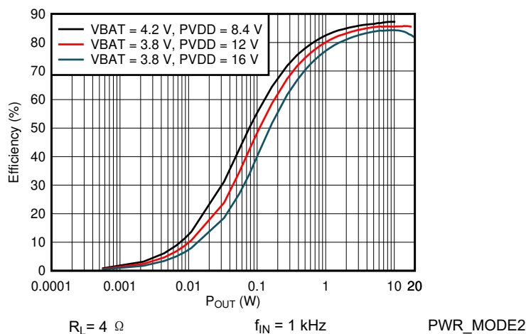
图 6-21. Efficiency vs Output Power
