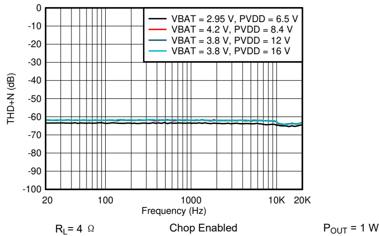
图 6-39. V Sense THDN vs Frequency
