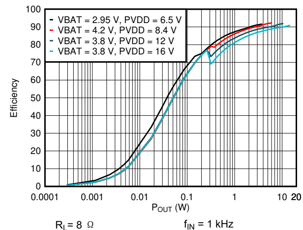
图 6-20. Efficiency vs Output Power
