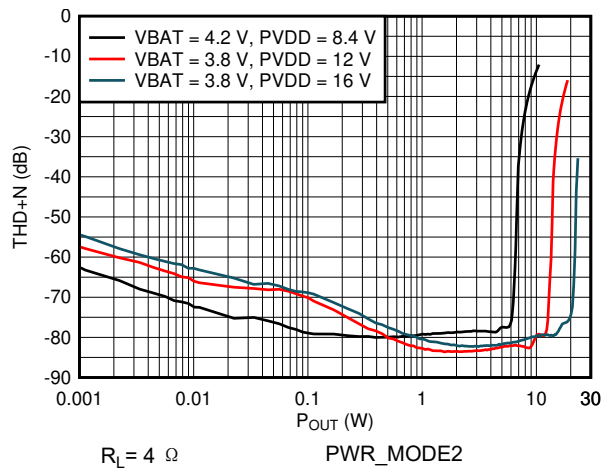
图 6-5. THD+N vs Output Power
