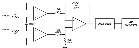
图 7-1. Differential To Single Ended (D2S) Filter
