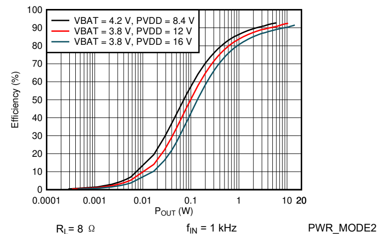
图 6-22. Efficiency vs Output Power
