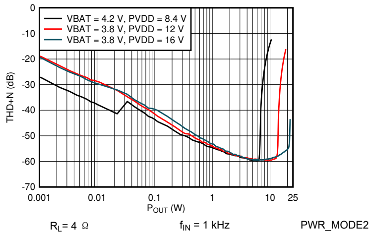
图 6-31. I Sense THDN vs Output Power
