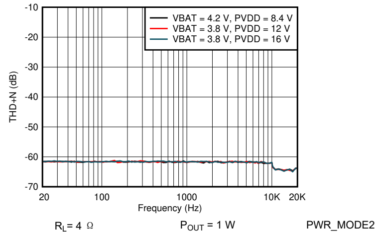
图 6-41. V Sense THDN vs Frequency
