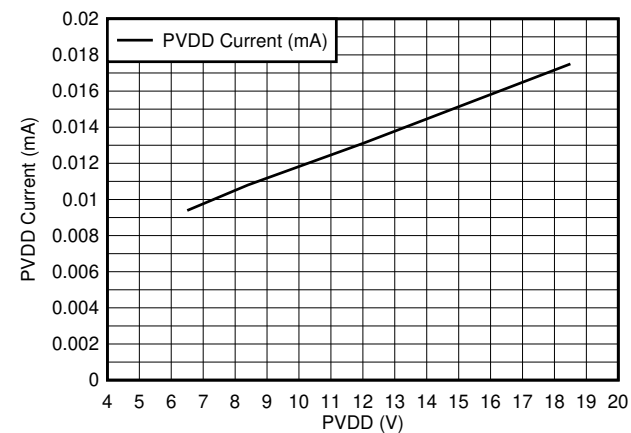
图 6-28. PVDD Idle Current vs PVDD
