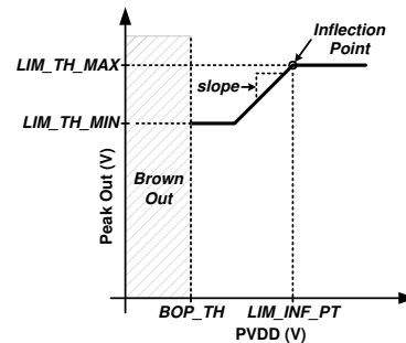
图 8-9. Limiter with Inflection Point and Minimum Threshold
