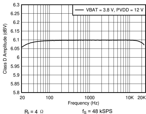
图 6-17. Class D Frequency Response
