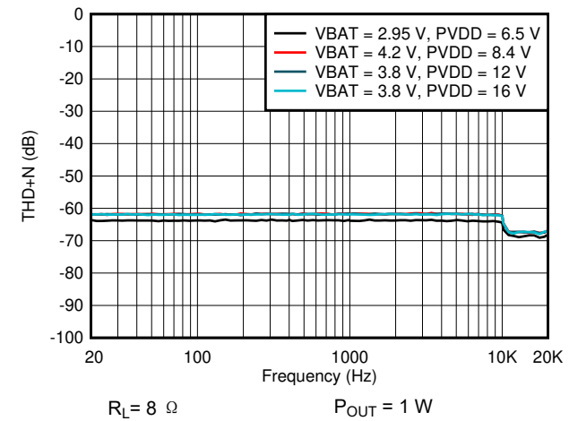
图 6-40. V Sense THDN vs Frequency
