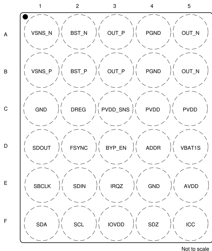
图 5-1. YBH Package 30-Ball DSBGA Top View
