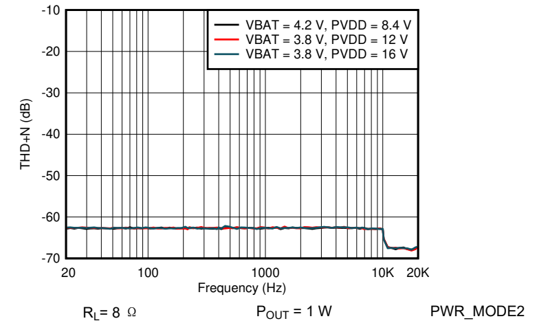
图 6-42. V Sense THDN vs Frequency
