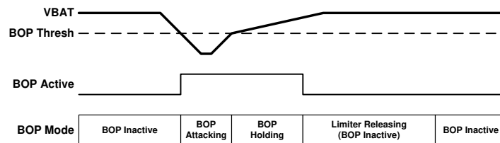
图 8-10. Brownout Prevention Event
