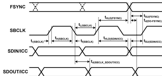
图 6-2. TDM and ICC Timing Diagram
