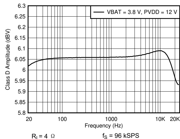
图 6-18. Class D Frequency Response
