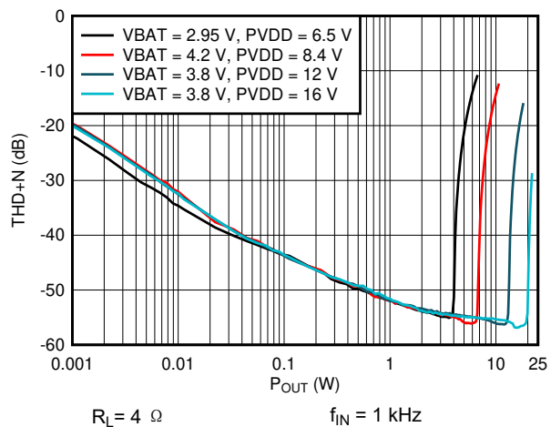
图 6-29. I Sense THDN vs Output Power
