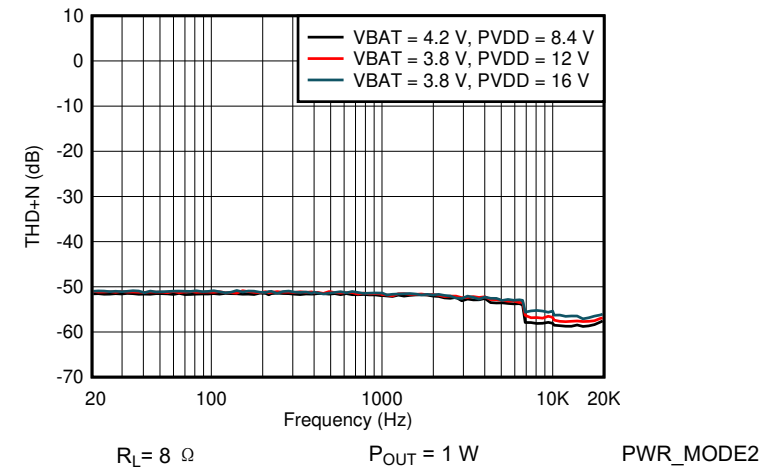
图 6-36. I Sense THD vs. Frequency
