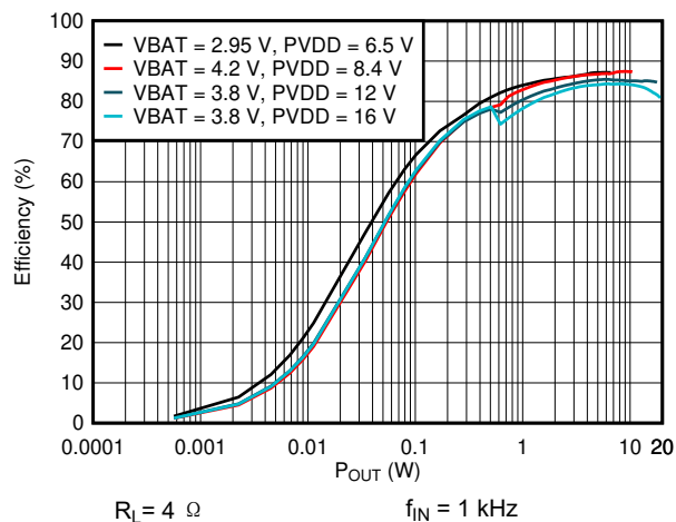
图 6-19. Efficiency vs Output Power
