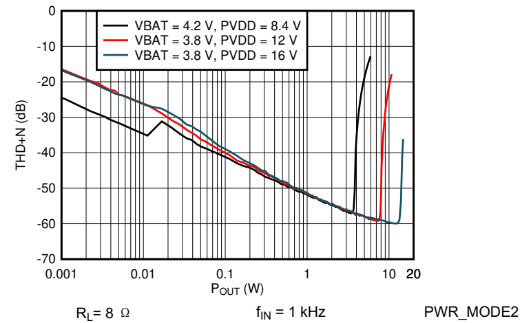
图 6-32. I Sense THDN vs Output Power
