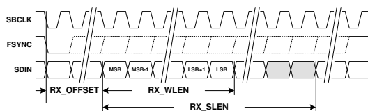
图 8-2. TDM RX Time Slot with Left Justification
