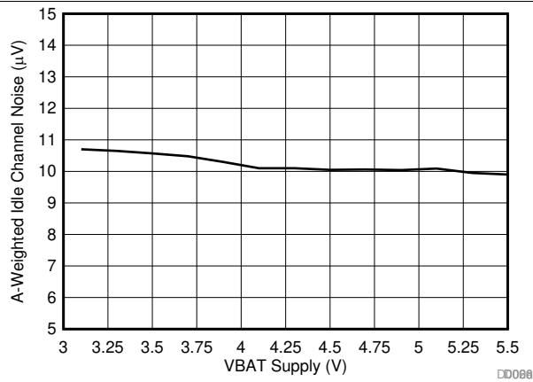
Figure 9. Receiver Idle Channel Noise (A-Weighted) vs VBAT
