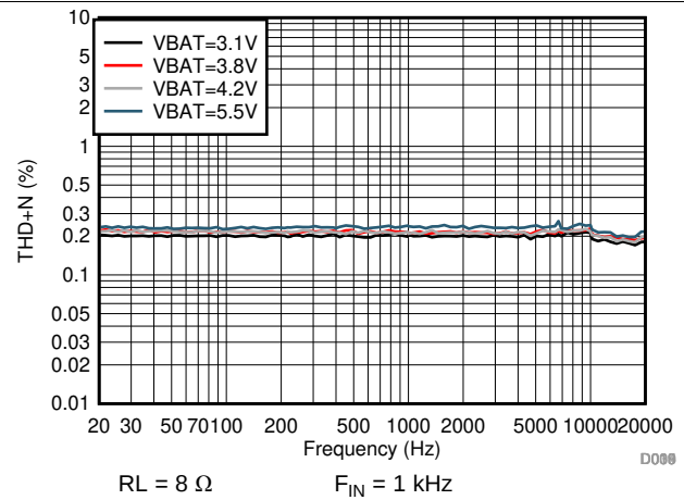
Figure 22. V-sense THD+N vs Frequency
