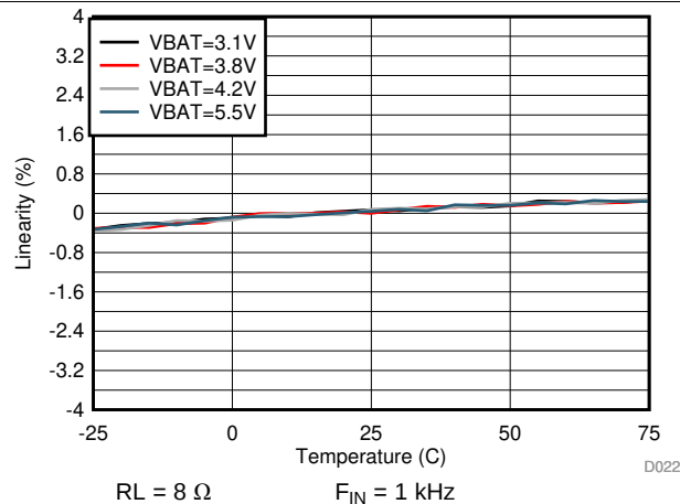
Figure 25. V-sense Linearity vs Temperature
