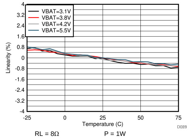
Figure 24. I-sense Linearity vs Temperature
