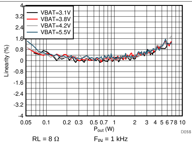
Figure 18. I-sense Linearity vs Output Power
