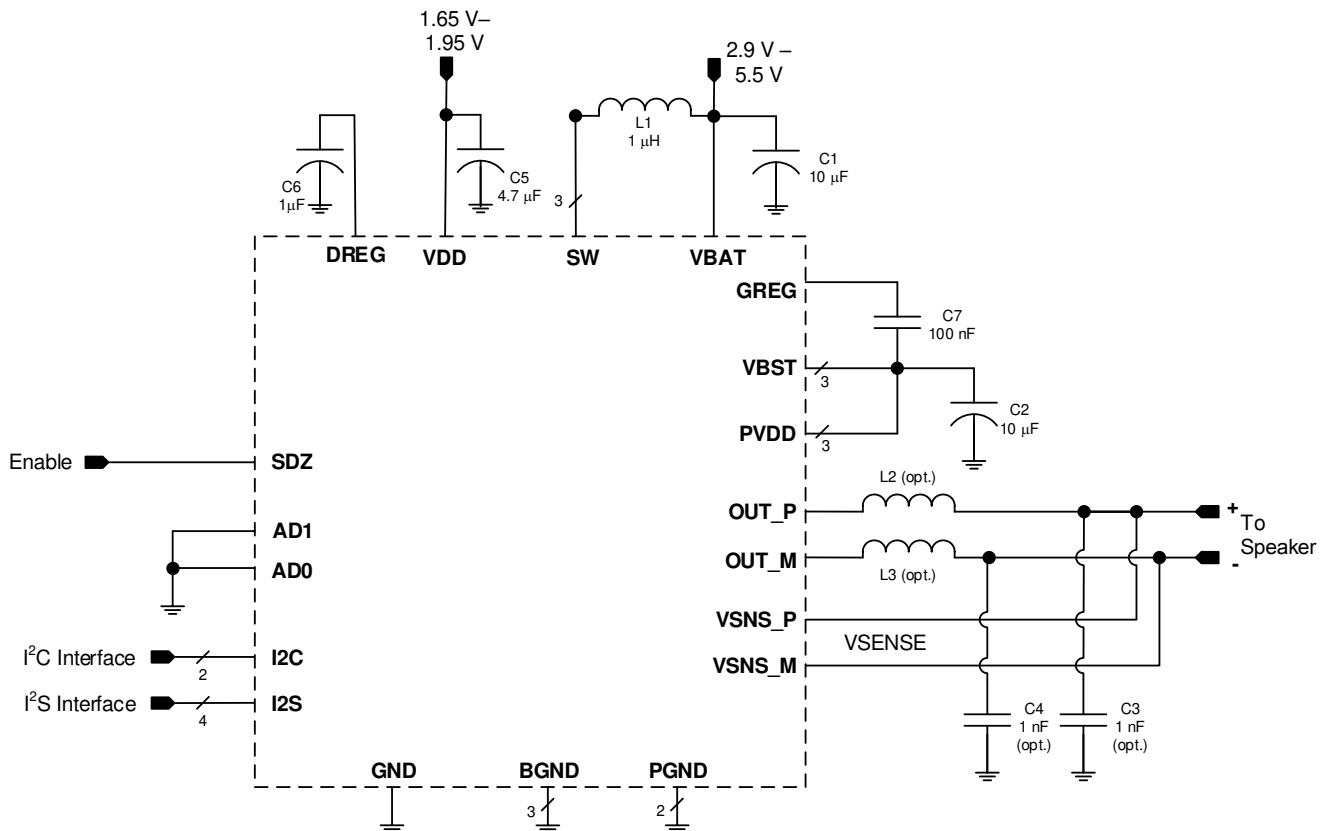
Figure 48. Typical Application - Digital Audio Input
