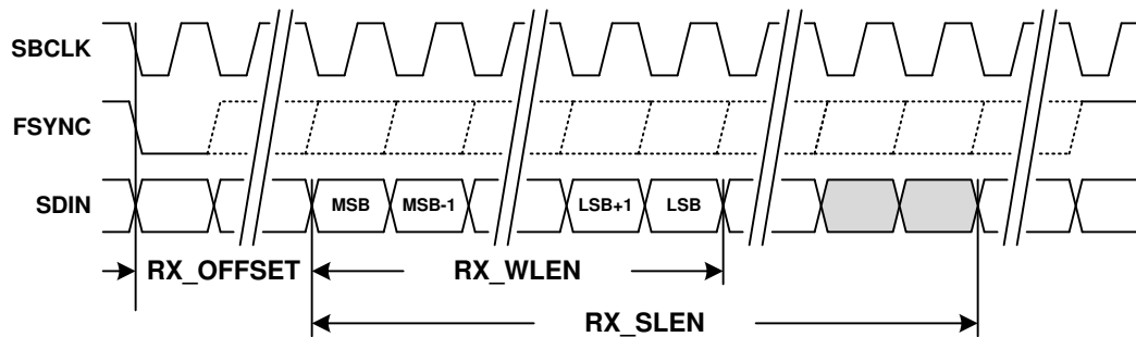
Figure 34. TDM RX Time Slot with Left Justification
