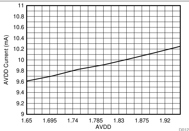
Figure 15. AVDD Idle Current vs AVDD
