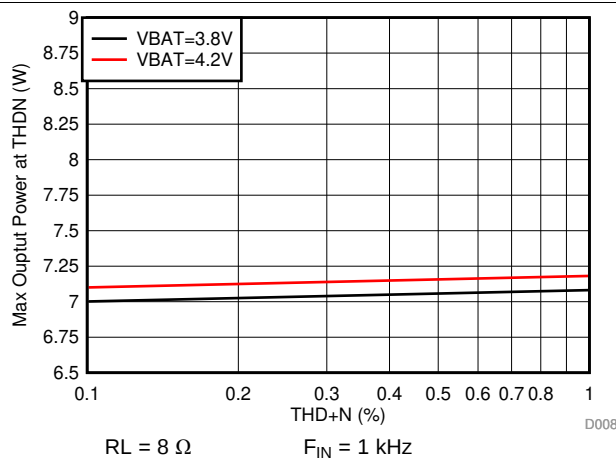
Figure 11. Max Output Power vs THD+N
