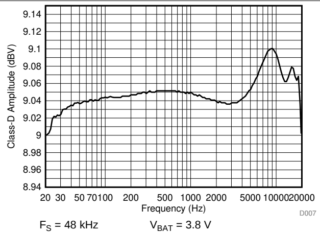
Figure 10. Amplitude vs Frequency
