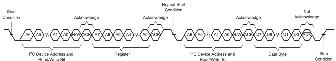
Figure 31. Single-Byte Read Transfer
