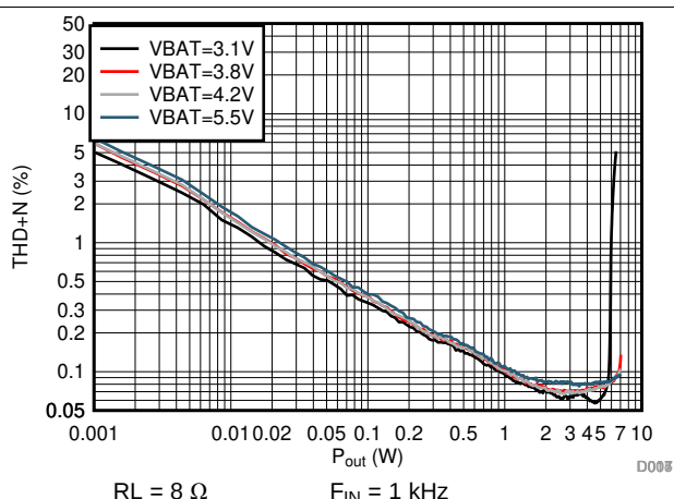
Figure 20. V-sense THD+N vs Output Power
