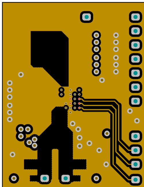
Figure 53. Second Copper Layer
