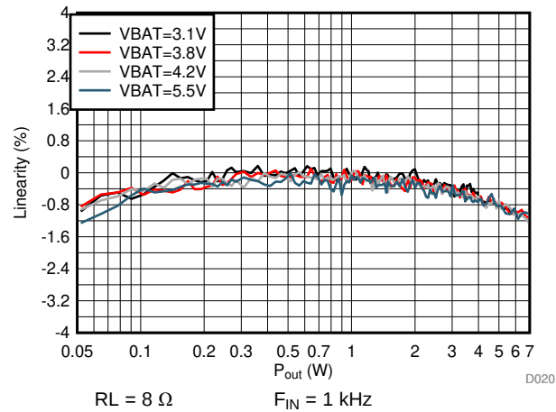
Figure 23. V/I-sense Linearity vs Output Power
