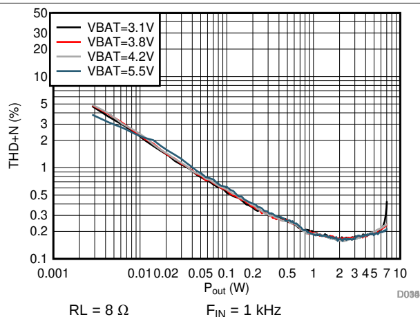
Figure 17. I-sense THD+N vs Output Power
