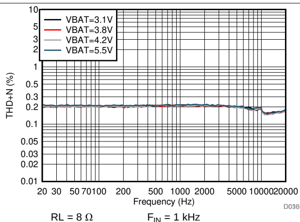
Figure 19. I-sense THD+N vs Frequency
