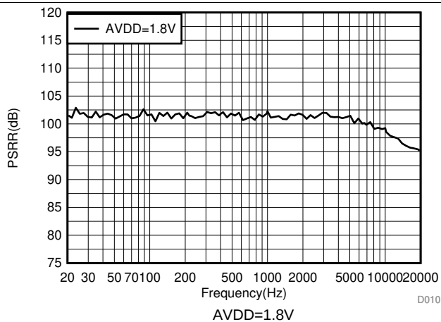
Figure 13. AVDD PSRR vs Frequency
