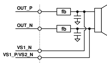
Figure 45. V-Sense Connections
