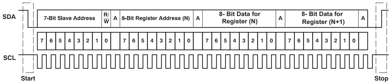
Figure 28. Typical I²C Sequence
