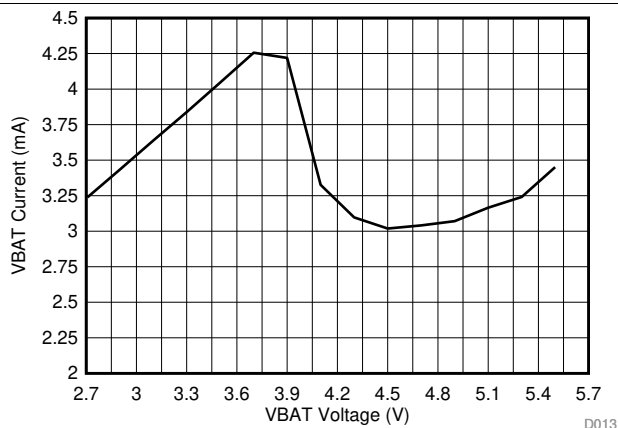
Figure 16. VBAT Idle Current vs VBAT
