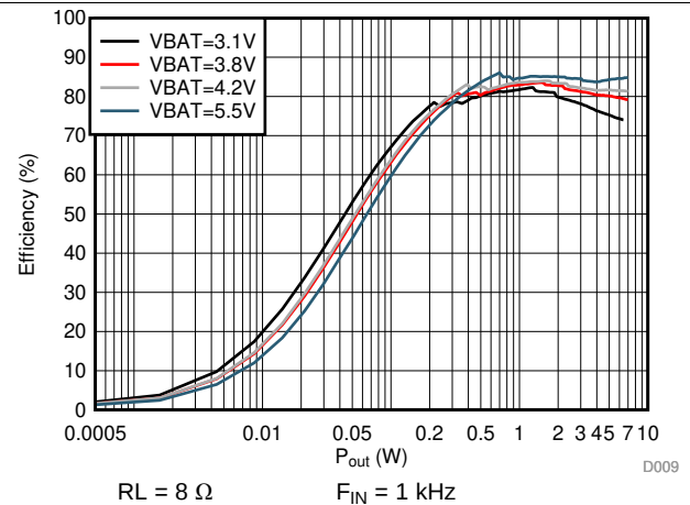
Figure 12. Efficiency vs Output Power
