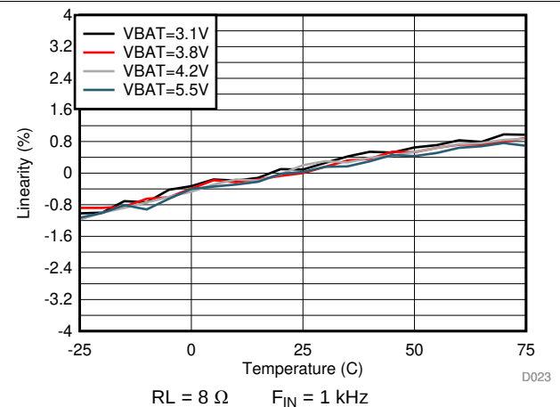
Figure 26. V/I-sense Linearity vs Temperature
