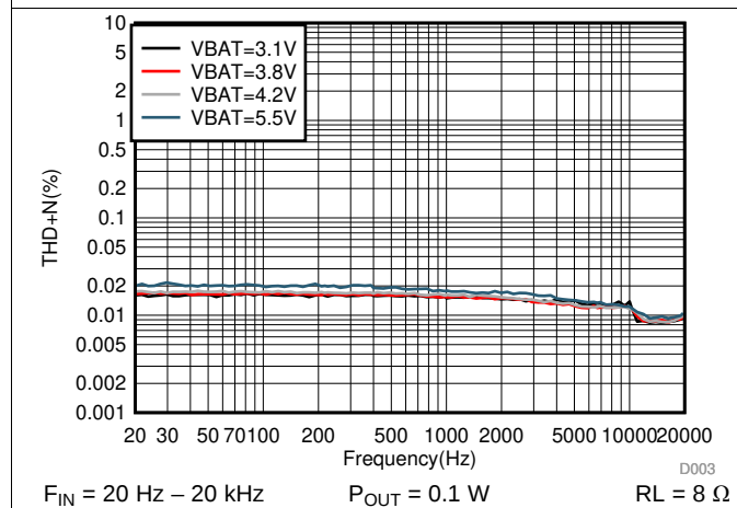
Figure 5. THD+N vs Frequency
