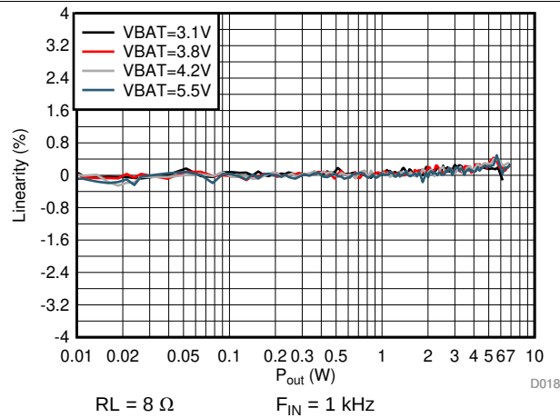
Figure 21. V-sense Linearity vs Output Power
