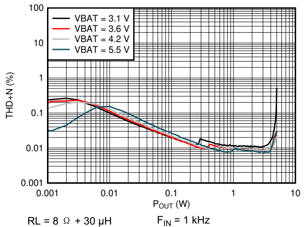
图 5-8. THD+N vs Output Power (QFN Package)
