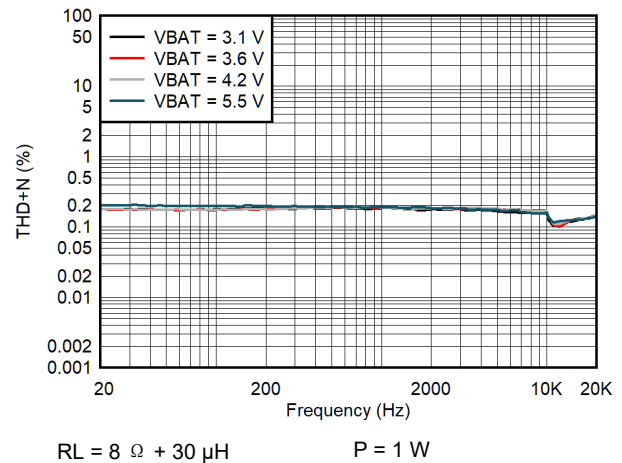
图 5-46. I-sense THD+N vs Frequency (QFN Package)
