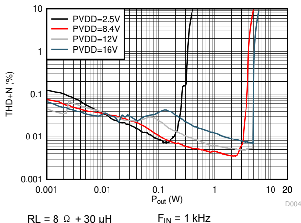
图 5-10. THD+N vs Output Power
