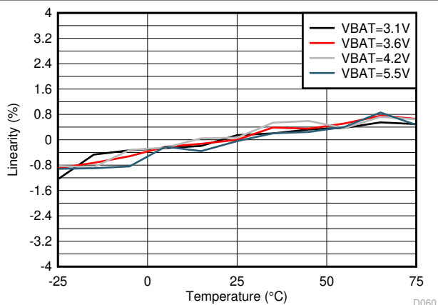
图 5-57. V/I-sense Linearity vs Temperature
