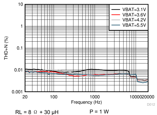
图 5-20. THD+N vs Frequency
