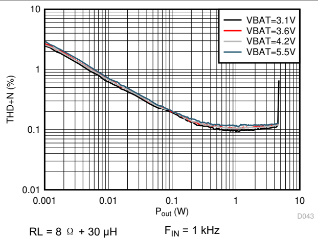
图 5-48. V-sense THD+N vs Output Power
