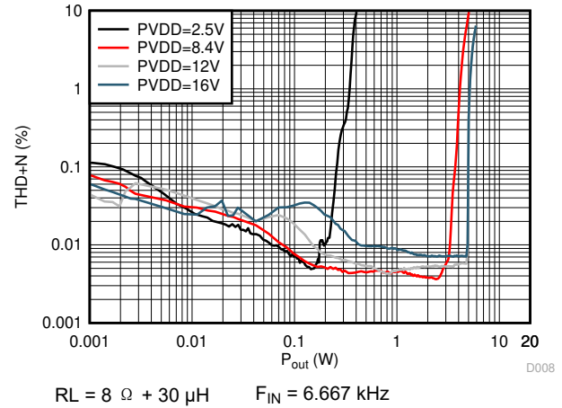
图 5-16. THD+N vs Output Power
