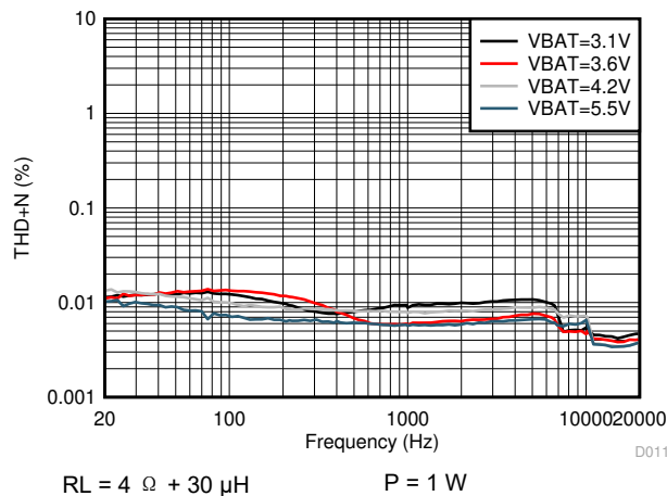
图 5-19. THD+N vs Frequency
