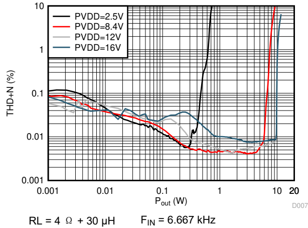
图 5-15. THD+N vs Output Power
