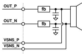
图 7-20. V-Sense Connections
