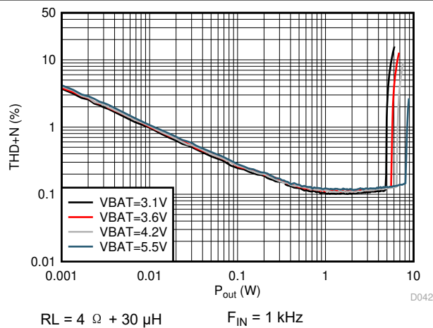
图 5-47. V-sense THD+N vs Output Power
