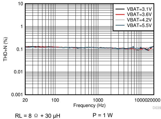
图 5-45. I-sense THD+N vs Frequency (DSBGA Package)
