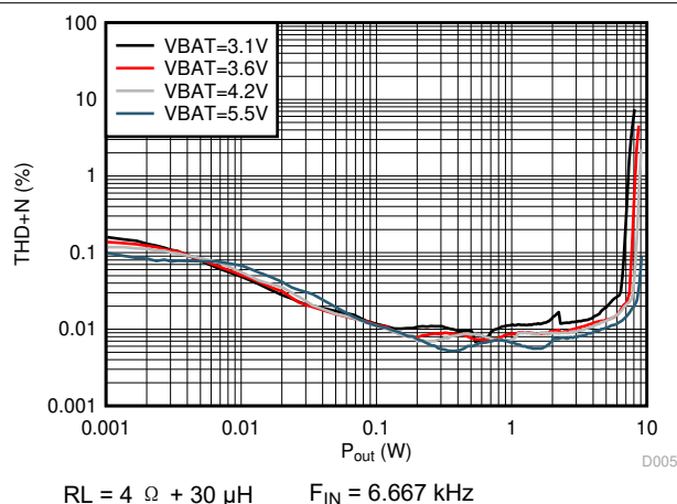
图 5-11. THD+N vs Output Power (DSBGA Package)
