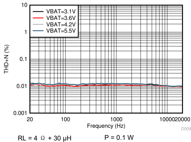
图 5-17. THD+N vs Frequency
