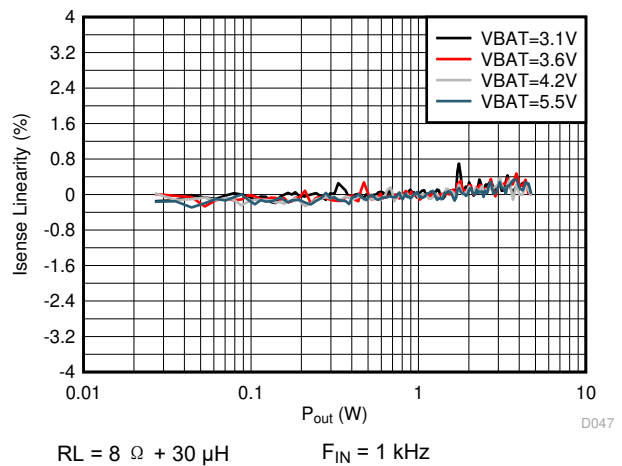
图 5-50. V-sense Linearity vs Output Power
