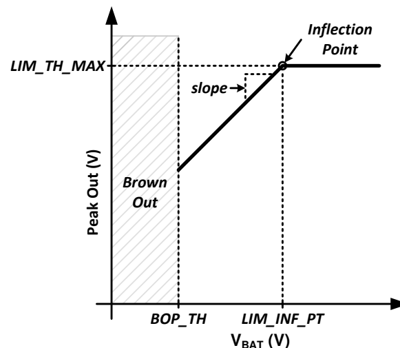
图 7-16. Limiter with Inflection Point
