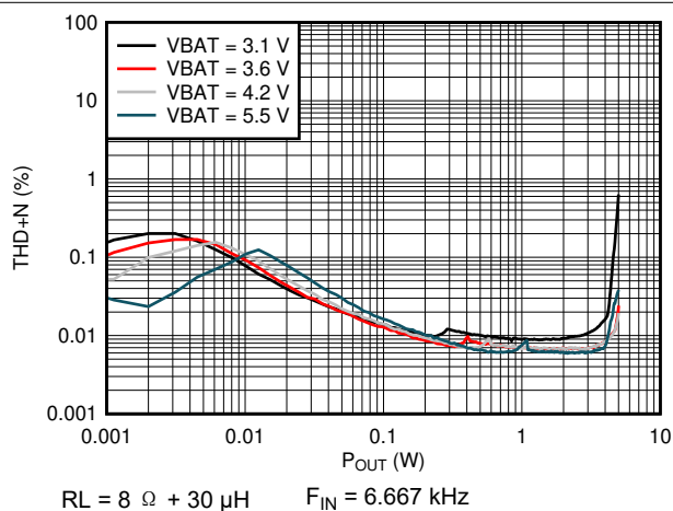
图 5-14. THD+N vs Output Power (QFN Package)
