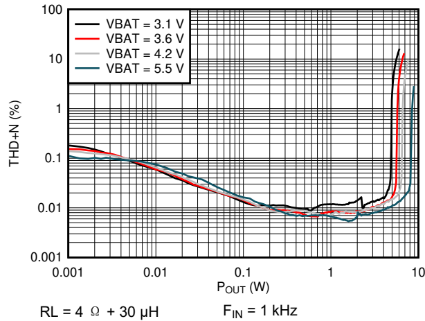
图 5-5. THD+N vs Output Power (DSBGA Package)
