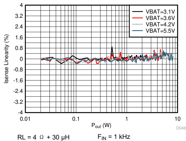
图 5-49. V-sense Linearity vs Output Power
