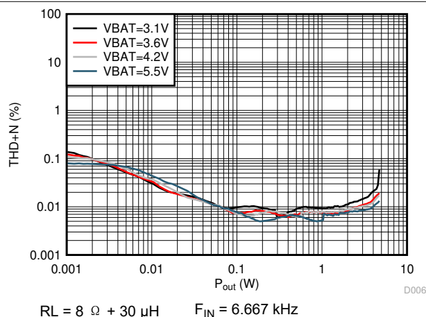
图 5-13. THD+N vs Output Power (DSBGA Package)
