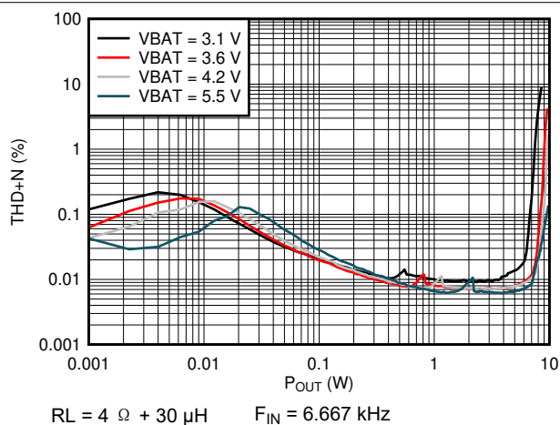
图 5-12. THD+N vs Output Power (QFN Package)
