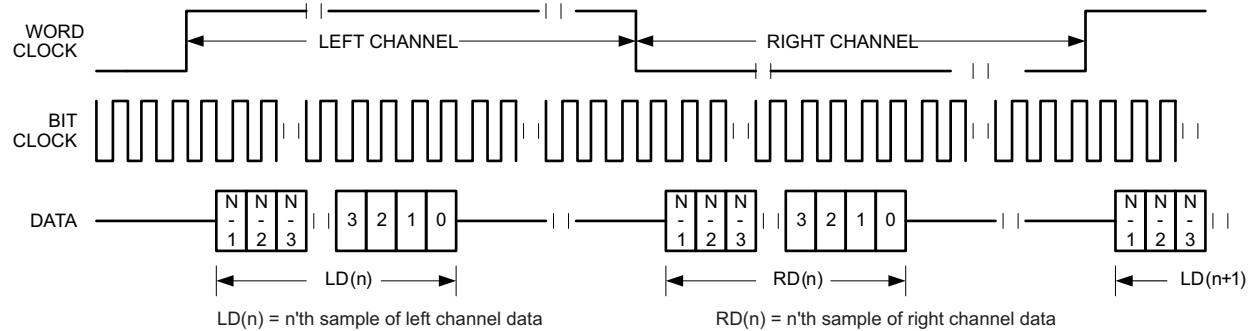
图 43. Timing Diagram for Left-Left Mode with ASI_OFFSET1 = 1
