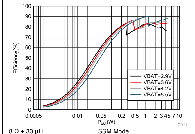
图 17. Efficiency vs Output Power High Efficiency
