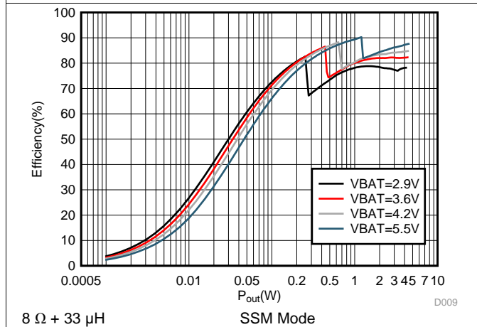
图 15. Efficiency vs Output Power Low Inrush
