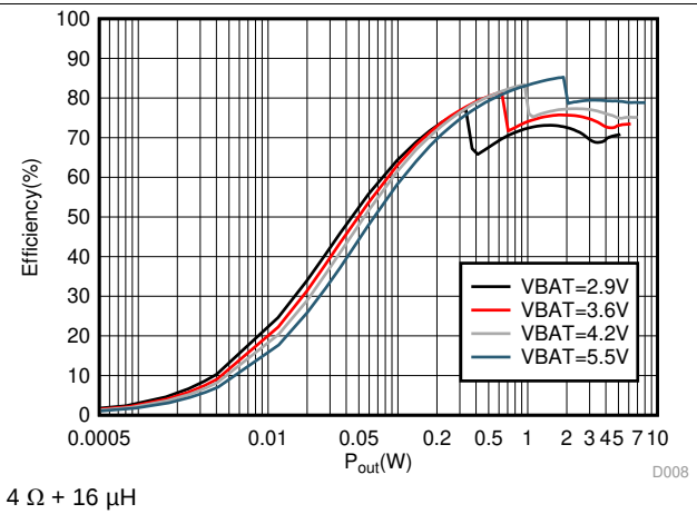
图 14. Efficiency vs Output Power
