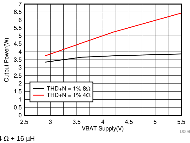
图 15. Output Power for 1% THD+N vs VBAT
