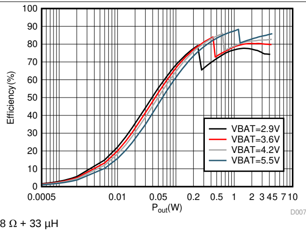
图 13. Efficiency vs Output Power
