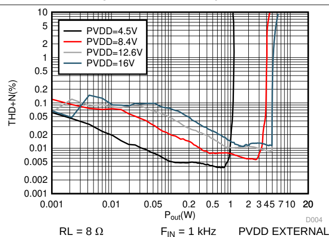
Figure 6. THD+N vs Output Power
