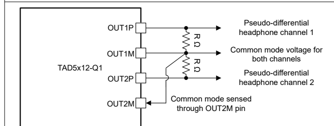
图 6-16. 带外部共模检测的伪差分输出连接 (OUT1x_CFG[2:0] = 3'b101)
