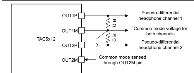
图 6-16. 带外部共模检测的伪差分输出连接 (OUT1x_CFG[2:0] = 3'b101)
