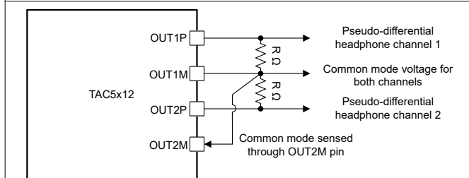
图 6-17. 带外部共模检测的伪差分输出连接 (OUT1x_CFG[2:0] = 3'b101)
