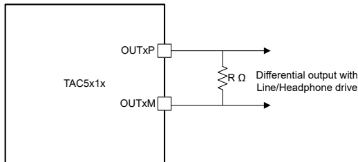
图 7-21. 差分输出连接 (OUT1x_CFG[2:0] = 3'b000)
