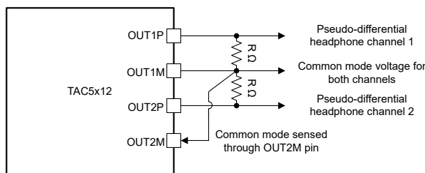
图 7-23. 带外部共模检测的伪差分输出连接 (OUT1x_CFG[2:0] = 3'b101)
