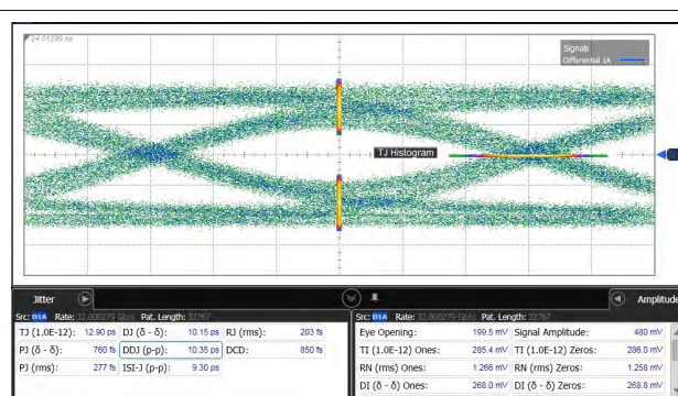
图 5-5. Through Calibration Trace (6.5dB Loss)
