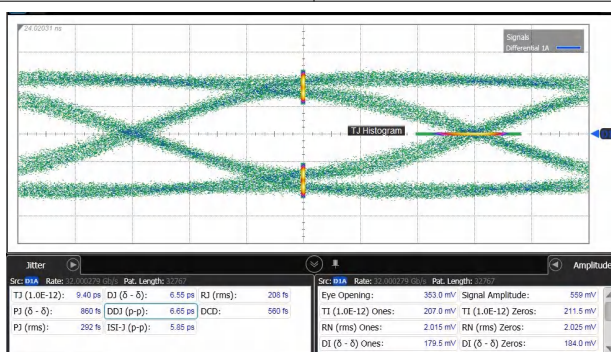
图 5-6. Through SN75LVPE5421 (6.5dB loss and DUT EQ=0)
