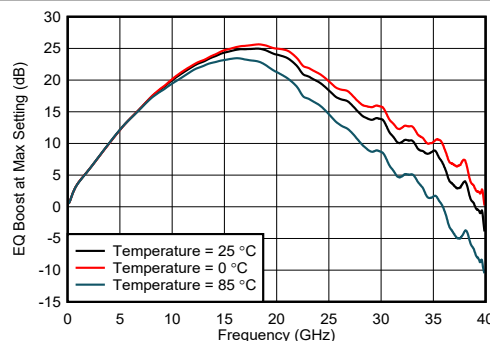
图 5-2. Typical EQ Boost vs Frequency at Different Temperature with EQ=19
