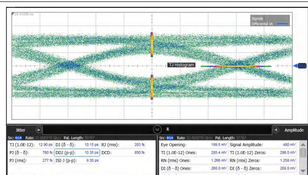
图 5-5. Through Calibration Trace (6.5dB Loss)
