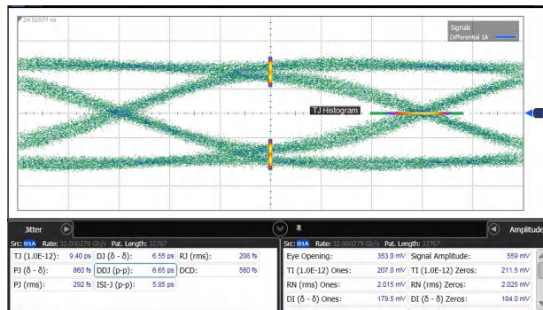
图 5-6. Through SN75LVPE5412 (6.5dB loss and DUT EQ=0)
