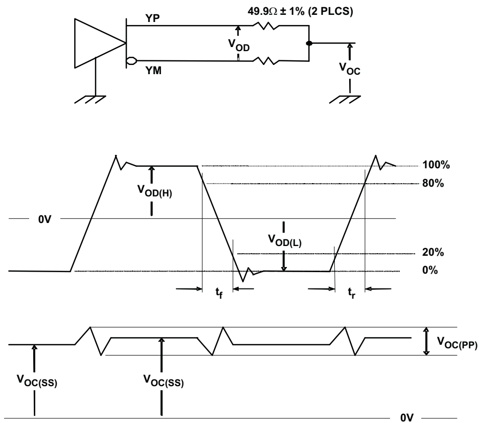
Figure 7. Test Load and Voltage Definitions for LVDS Outputs
