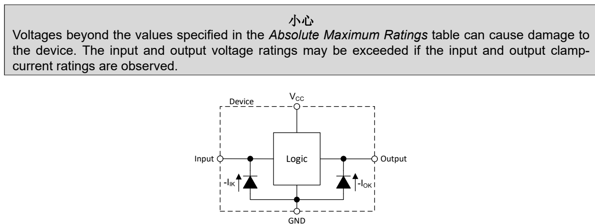
图 7-1. Electrical Placement of Clamping Diodes for Each Input and Output
