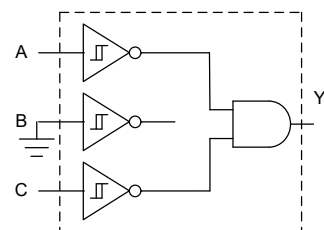
2 - Input AND Gate
