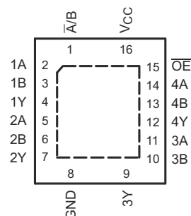
图 3-2. BQB Package, 16-Pin WQFN with Exposed Thermal Pad (Top View)
