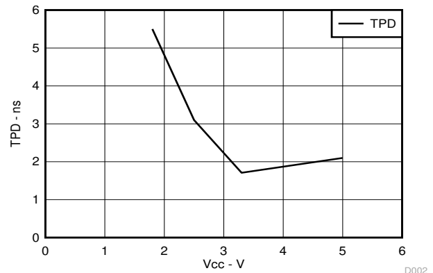
Figure 5-2. TPD Across V_{CC} at 25°C
