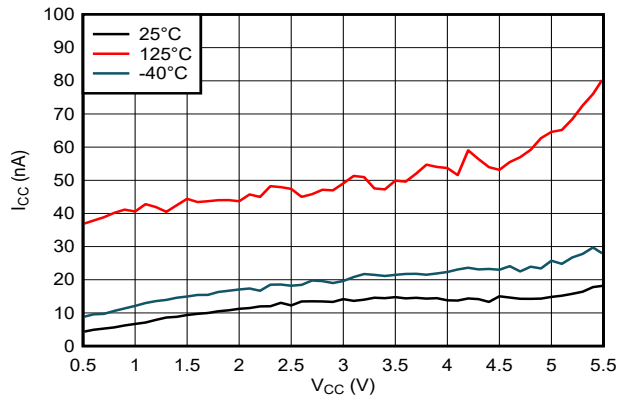
图 6-1. Supply Current Across Operating Voltage
