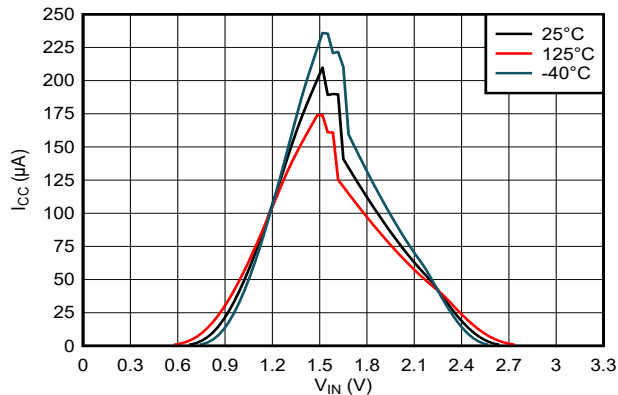
图 6-3. Supply Current Across Input Voltage, 3.3-V Supply
