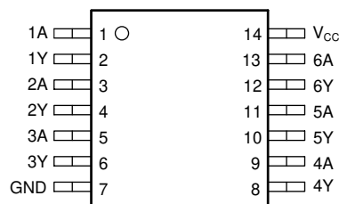
图 5-2. SN74LV6T14 PW Package, 14-Pin TSSOP (Top View)
