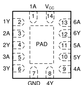
图 5-1. SN74LV6T06-Q1 BQA Package, 14-Pin WQFN (Top View)
