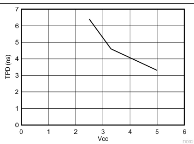
图 6-3. TPD vs. Vcc at 25°C
