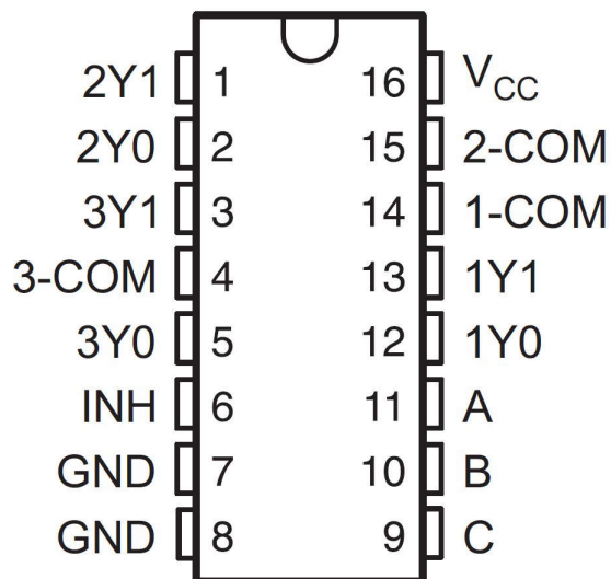
图 4-1. D, PW or DYY Package, 16-Pin TSSOP, SOT-23-THIN (Top View)
