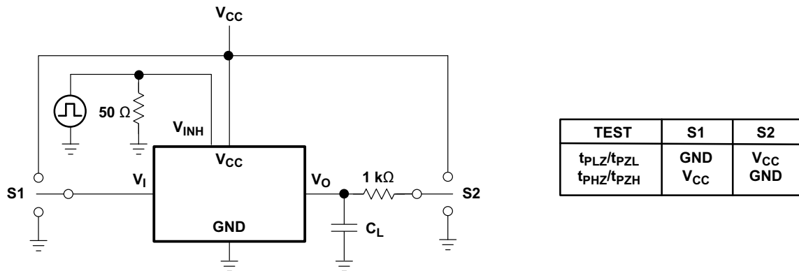
TEST CIRCUIT
