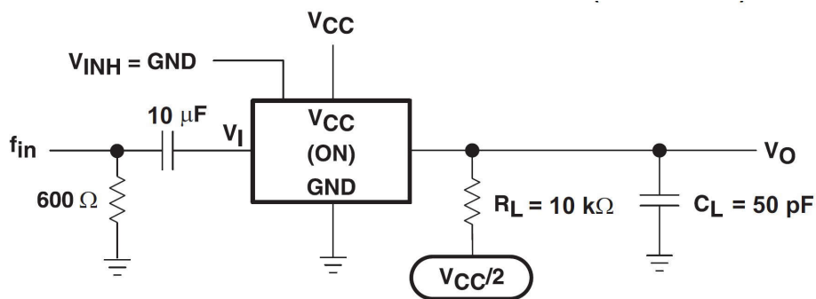
图 6-10. Sine-Wave Distortion
