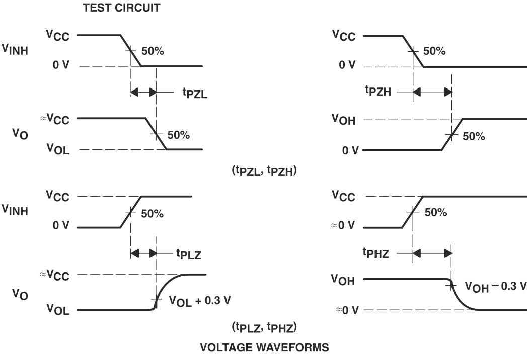
图 6-5. Switching Time ( t_{PZL} , t_{PLZ} , t_{PZH} , t_{PLH} ), Control to Signal Output
