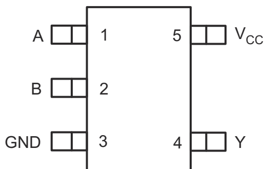
图 4-1. SN74LV1T32-Q1 DBV Package, 5-Pin SOT-23; DCK Package, 5-Pin SC-70 (Top View)
