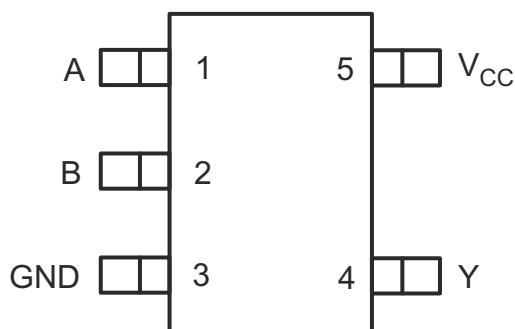
图 4-1. SN74LV1T00-Q1 DBV Package, 5-Pin SOT-23; DCK Package, 5-Pin SC-70 (Top View)
