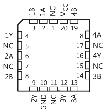
SN54LV132A: FK Package (Top View)
