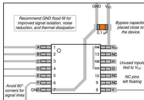
Figure 11. Example layout for the SN74HCS30
