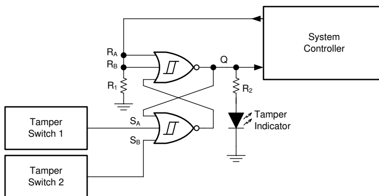
图 9. Typical application block diagram
