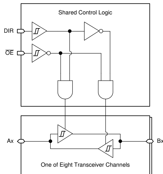
图 8-1. Logic Diagram (Positive Logic) for SN74HCS245-Q1
